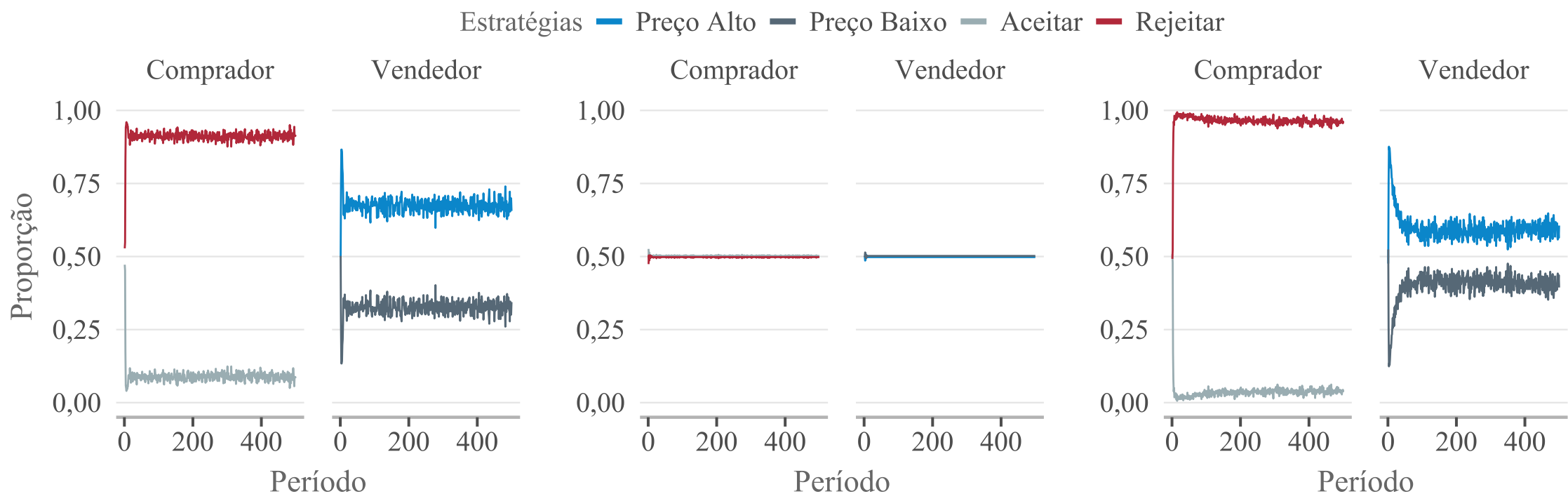
(a) EWA – BSG ( \lambda = 1 )
