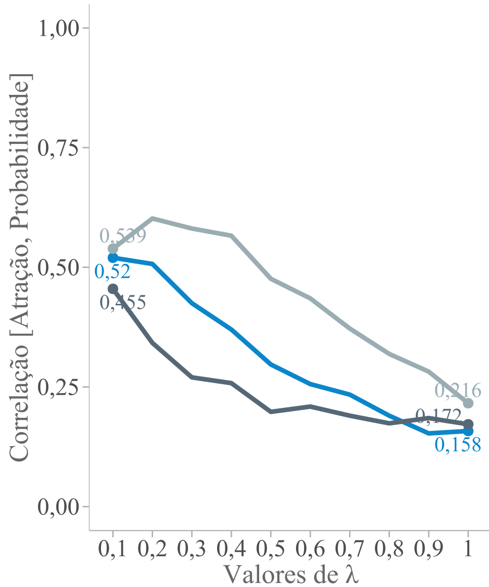
(a) BSG
