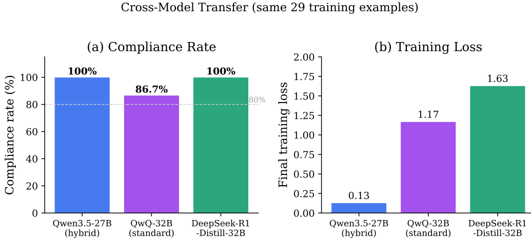
Figure 8: Within-family transfer using identical training data. All three models share Qwen-family base weights.
