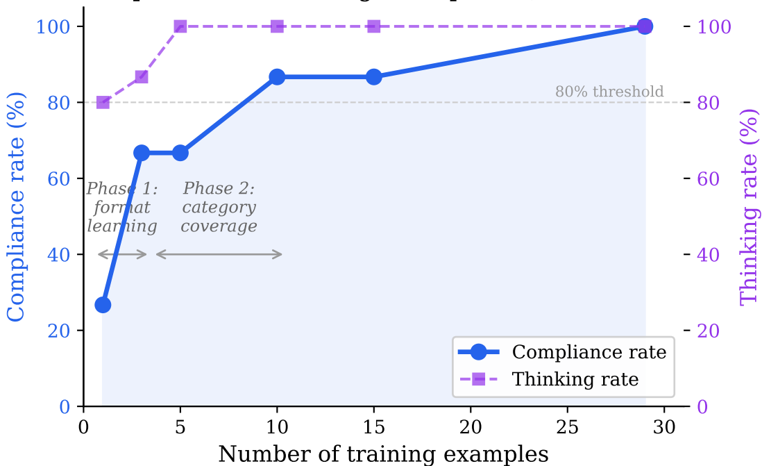
Compliance vs. Training Examples (Qwen3.5-27B)
