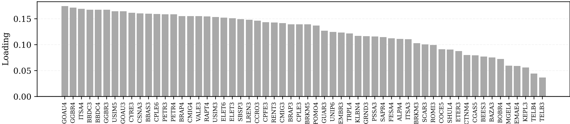
Eigenvector 1 ( \lambda = 21.65 ) | Market Mode
