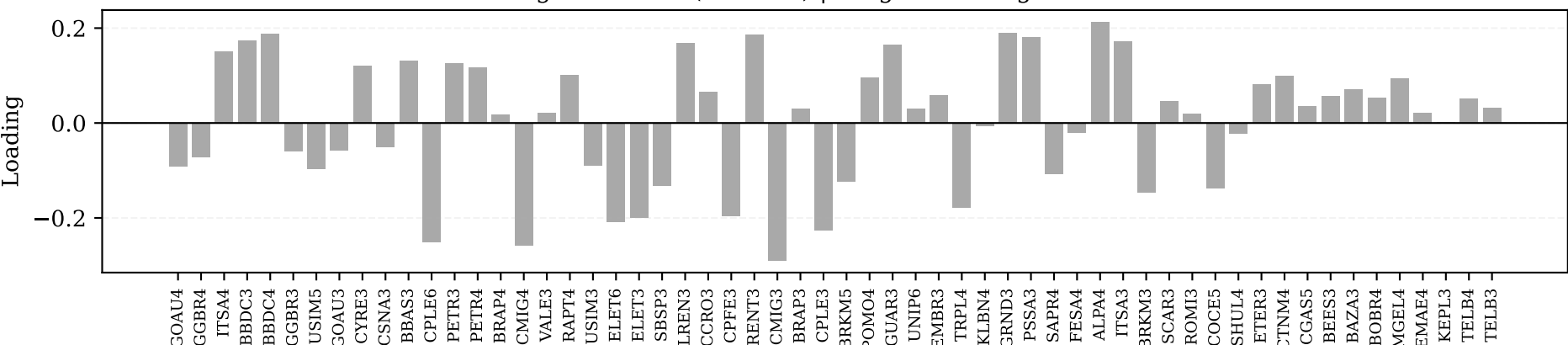
Eigenvector 5 ( \lambda = 1.48 ) | Largest loadings: Utilities
