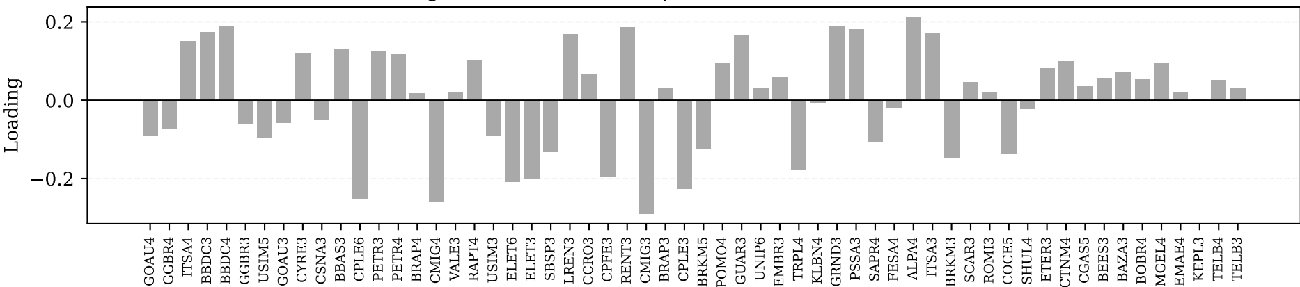
Eigenvector 5 ( \lambda = 1.48 ) | Utilities versus mixed sectors
