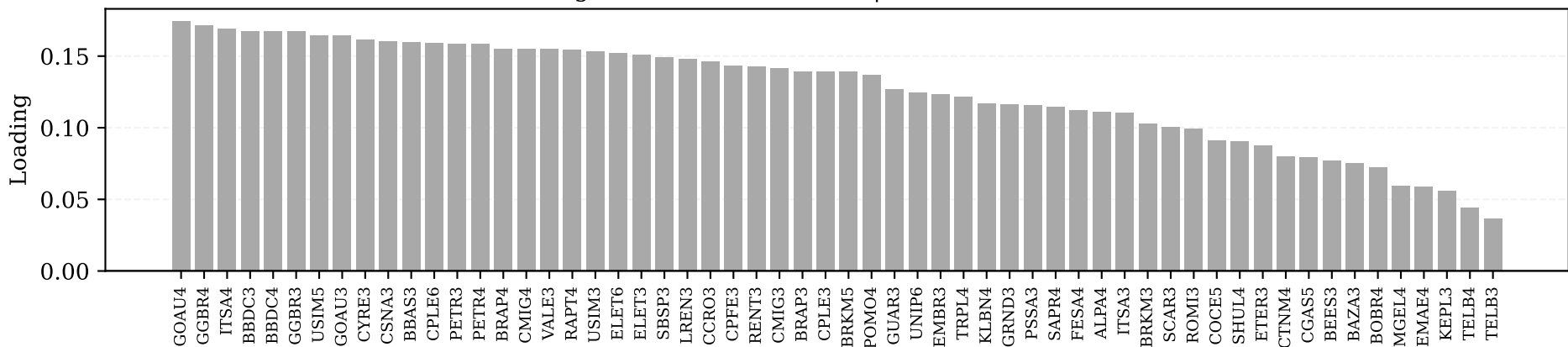
Eigenvector 1 ( \lambda = 21.65 ) | Market-wide mode
