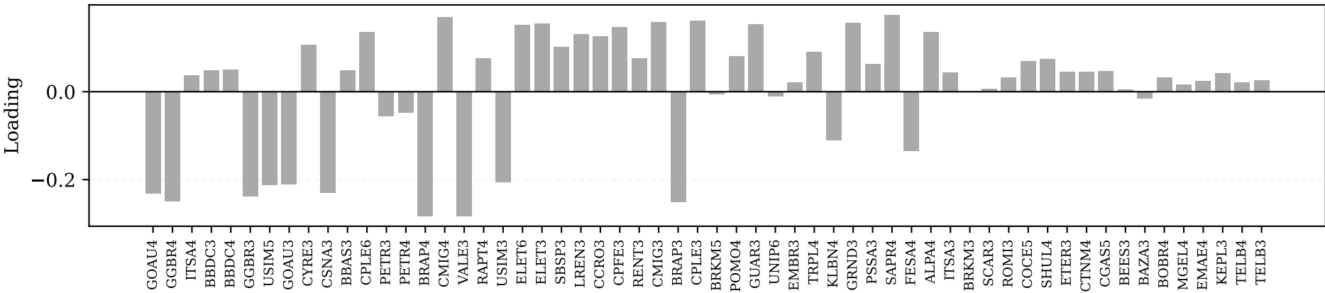
Eigenvector 3 ( \lambda = 1.78 ) | Financials versus industrial/consumer
