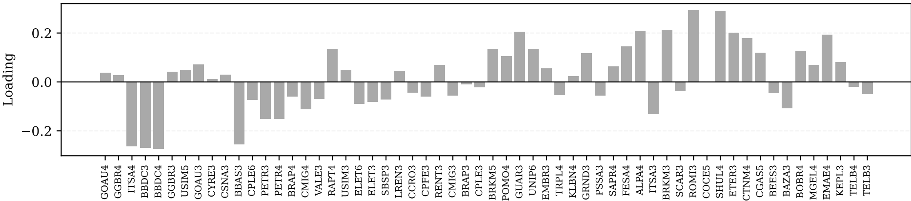
Eigenvector 4 ( \lambda = 1.65 ) | TELEBRAS share-class component
