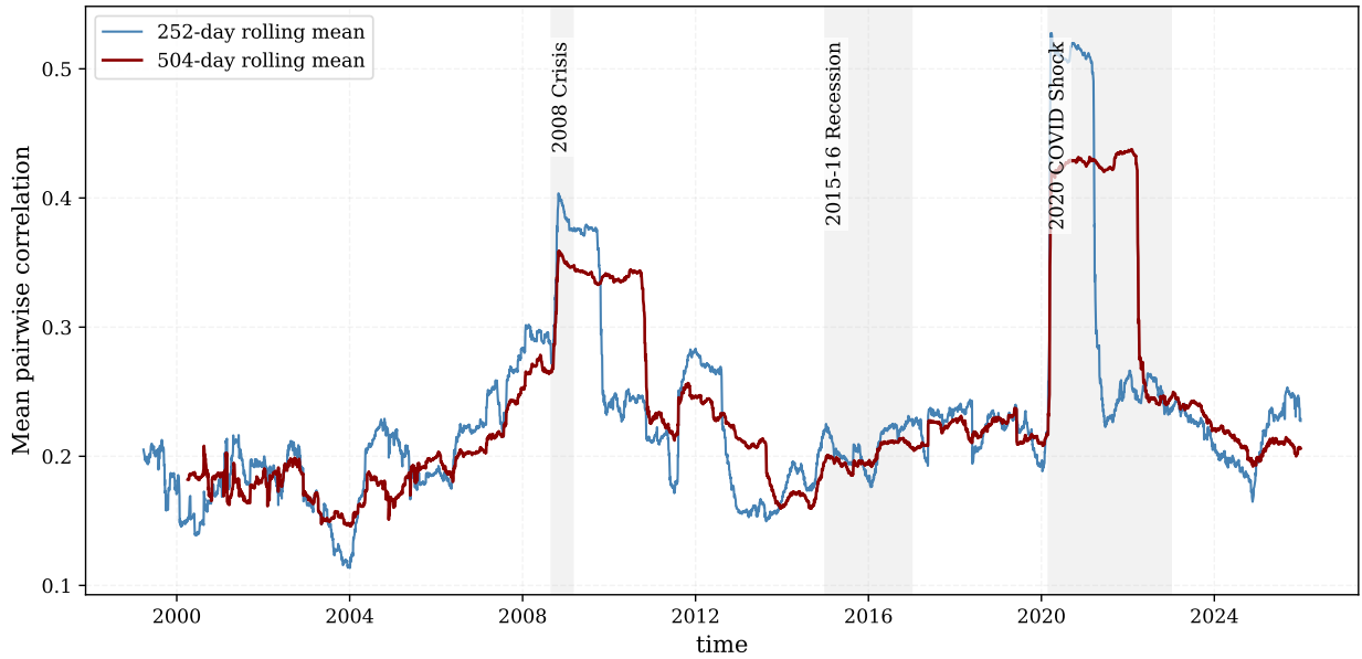
Figure 4: Rolling average market correlation for the core historical universe.
