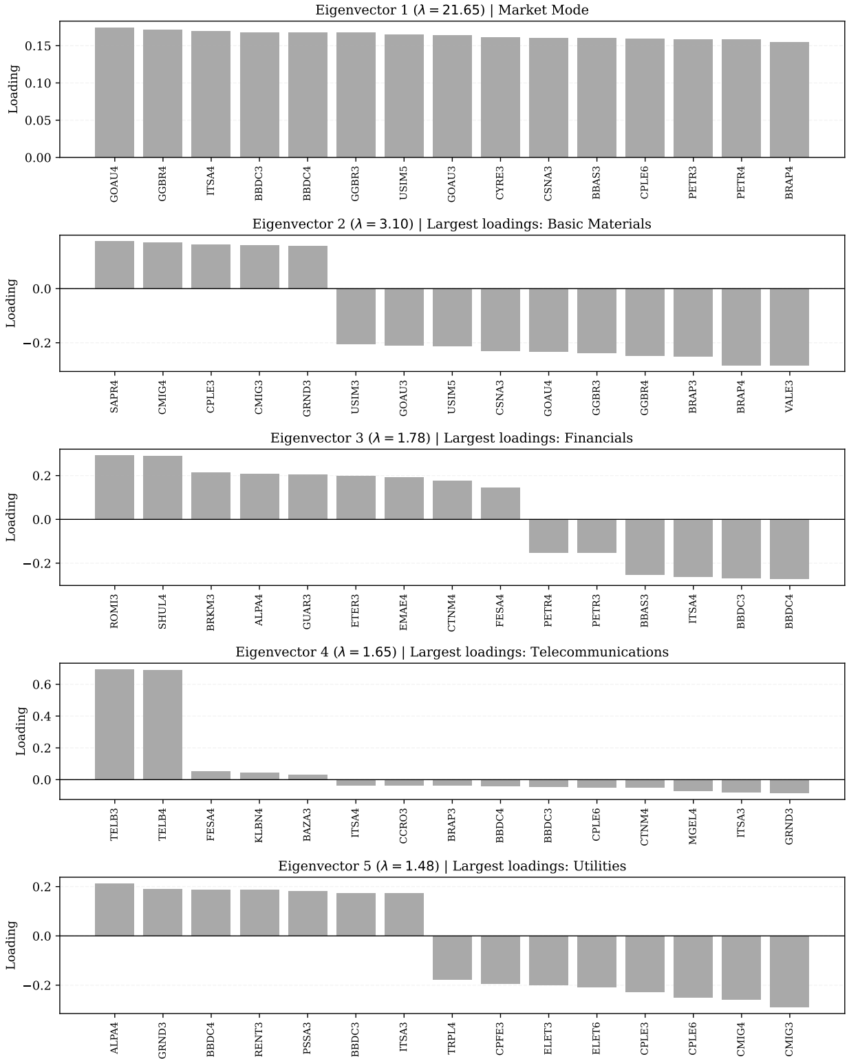
Figure 8: Top eigenvector loadings for the leading RMT modes. Eigenvector 1 captures the market-mode component; subsequent eigenvectors are read as candidate group or localized sectoral components.
