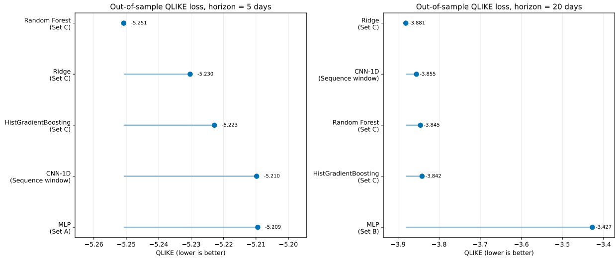
Figure 16: Volatility forecasting comparison for machine-learning and deep-learning models. Labels show the validation-selected feature set for each model and horizon.
