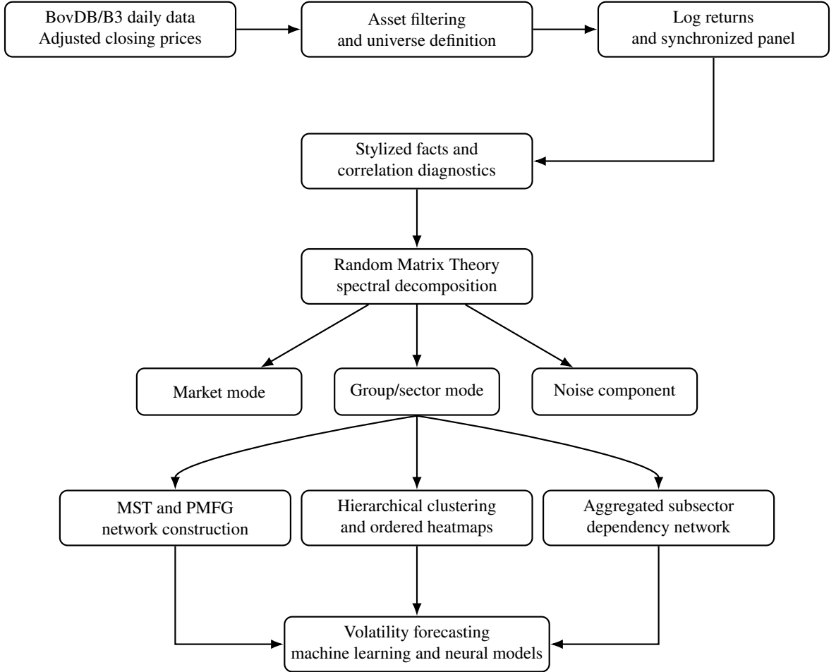
Figure 1: Overview of the empirical workflow. Adjusted daily B3 prices are filtered to define the equity universe and construct synchronized return panels. The workflow proceeds through stylized-fact checks, correlation estimation, Random Matrix Theory filtering, hierarchical clustering, MST/PMFG network construction, subsector aggregation and volatility forecasting with machine-learning, deep-learning, RMT and network-based features.
