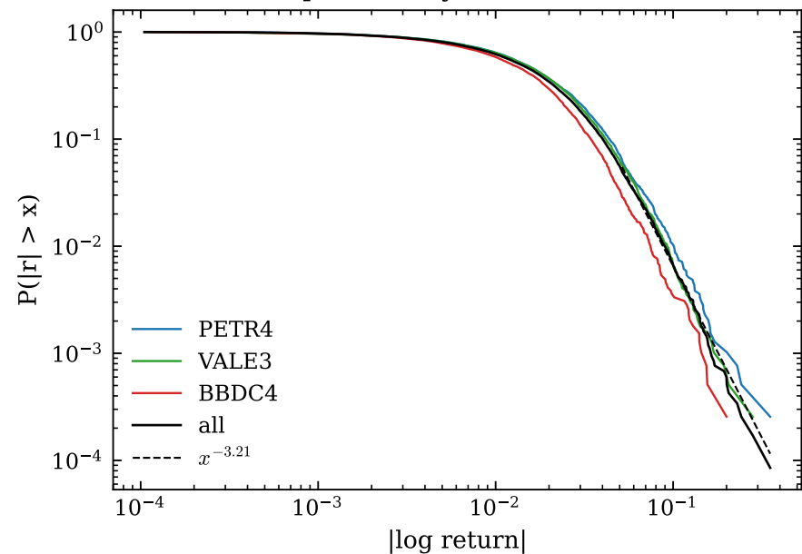
complementary CDF of returns
