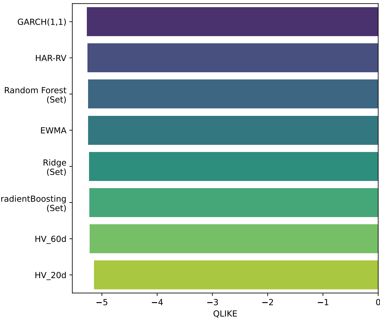
Out-of-Sample QLIKE Loss (Horizon = 5d)
