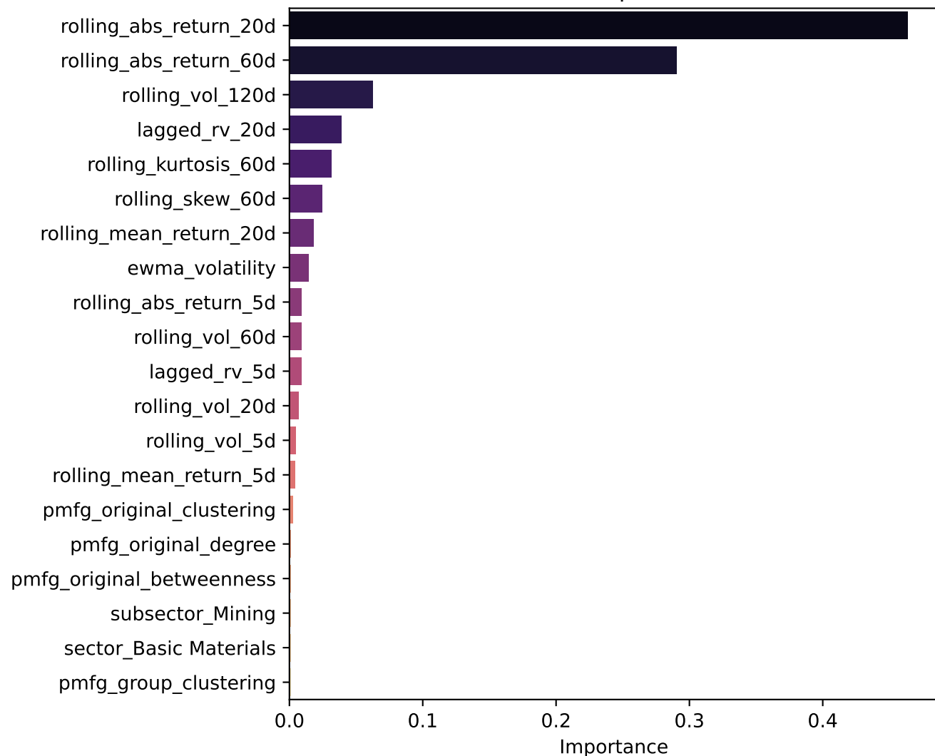
Random Forest Feature Importance (Horizon = 20d)
