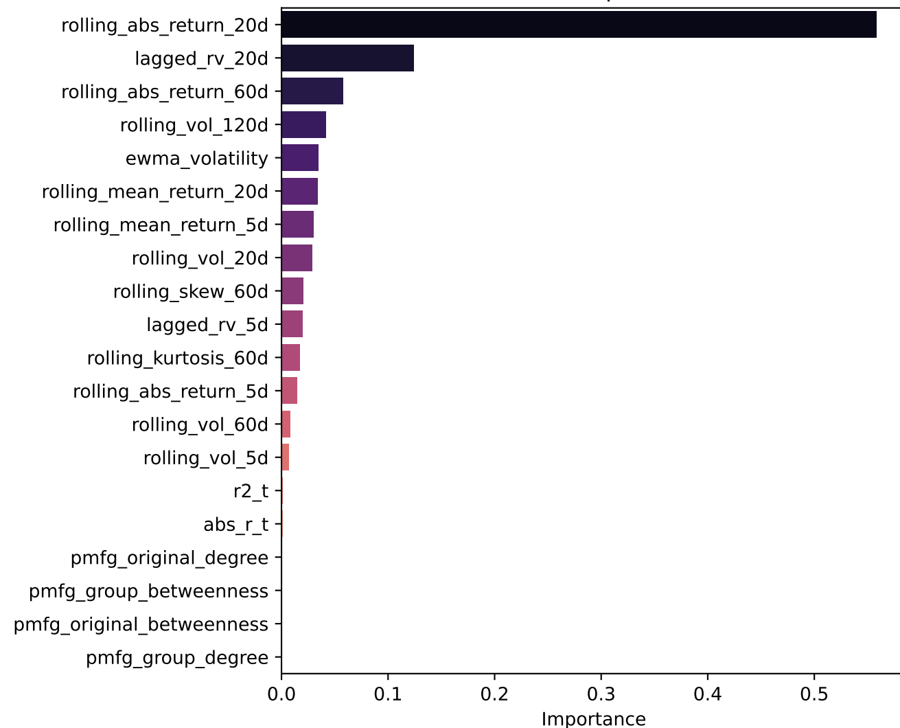
Random Forest Feature Importance (Horizon = 5d)
