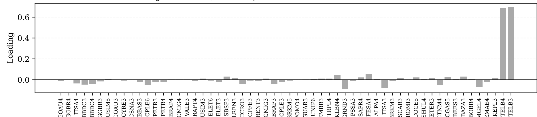
Eigenvector 4 ( \lambda = 1.65 ) | Dominant Sector: Telecommunications
