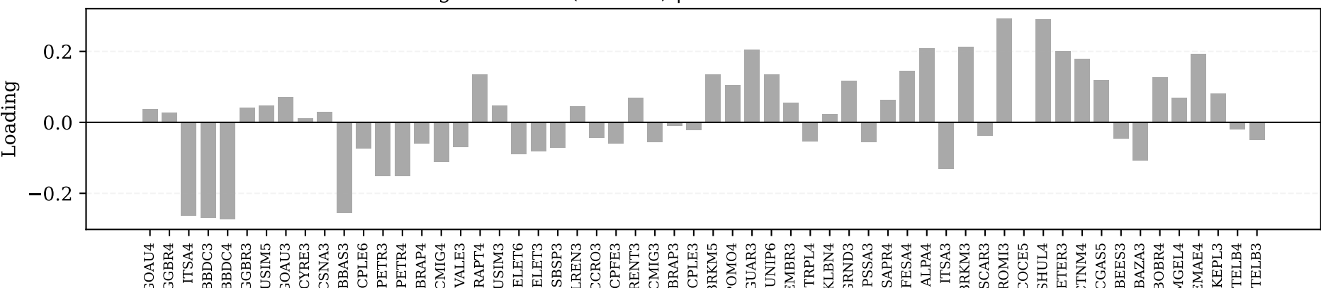
Eigenvector 3 ( \lambda = 1.78 ) | Dominant Sector: Financials
