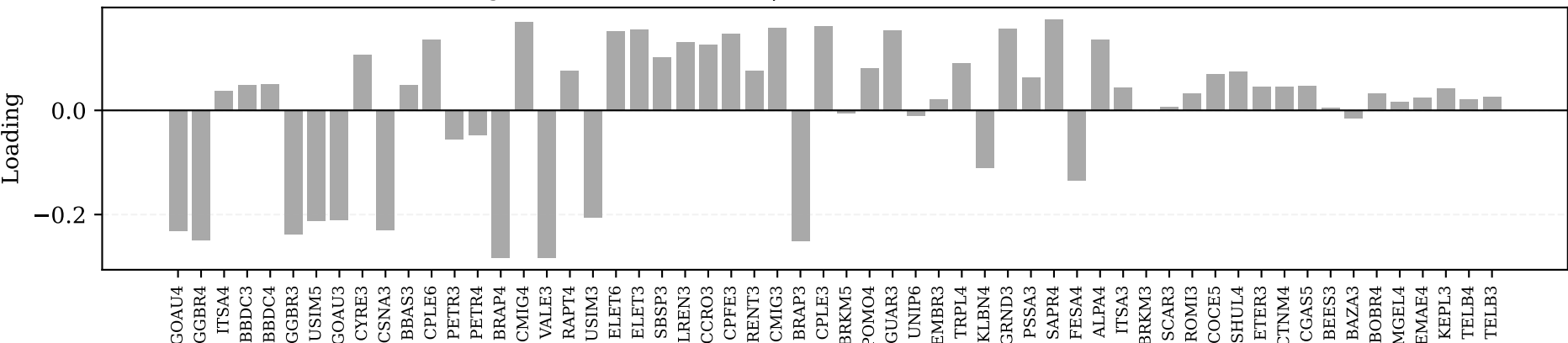
Eigenvector 2 ( \lambda = 3.10 ) | Dominant Sector: Basic Materials
