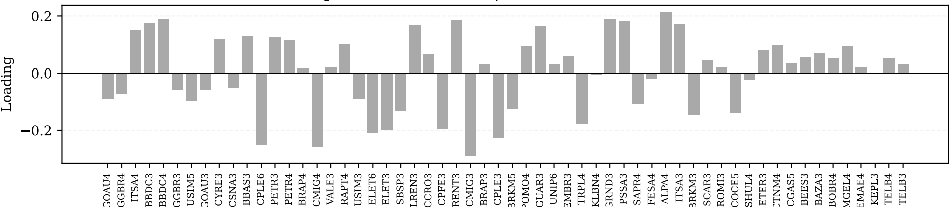
Eigenvector 5 ( \lambda = 1.48 ) | Dominant Sector: Utilities
