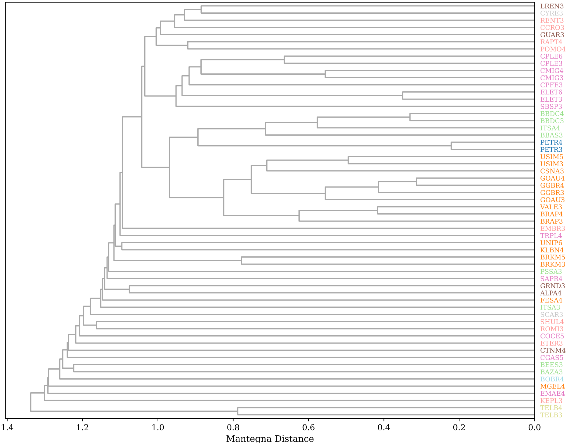
Filtered Correlation Matrix Dendrogram (UPGMA)
