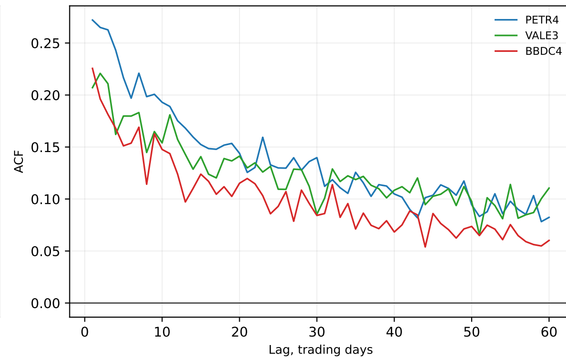
Autocorrelation of absolute returns
