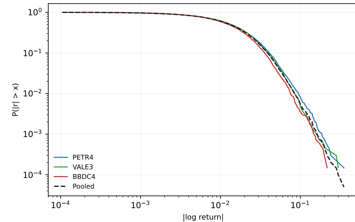
CCDF of absolute returns
