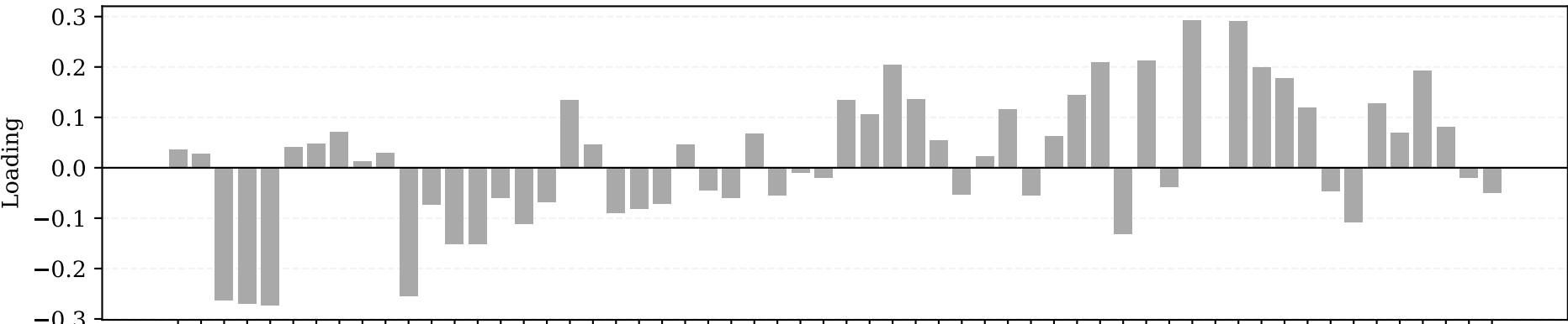
Eigenvector 3 ( \lambda = 1.78 ) | Dominant Sector: Financials
