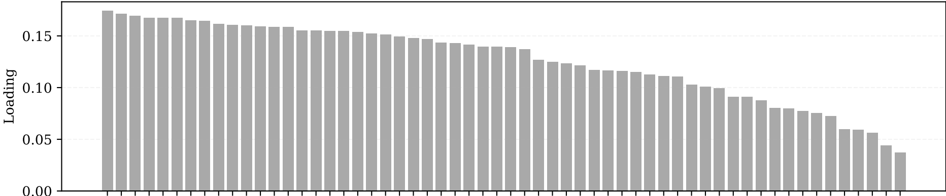
Eigenvector 1 ( \lambda = 21.65 ) | Dominant Sector: Basic Materials
