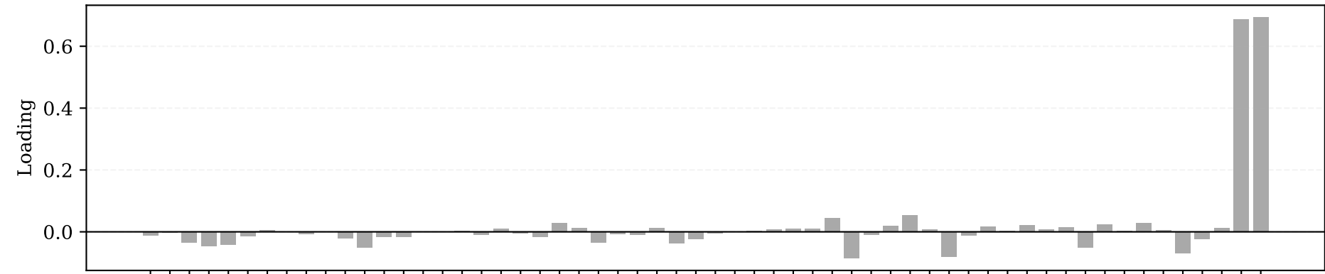
Eigenvector 4 ( \lambda = 1.65 ) | Dominant Sector: Telecommunications
