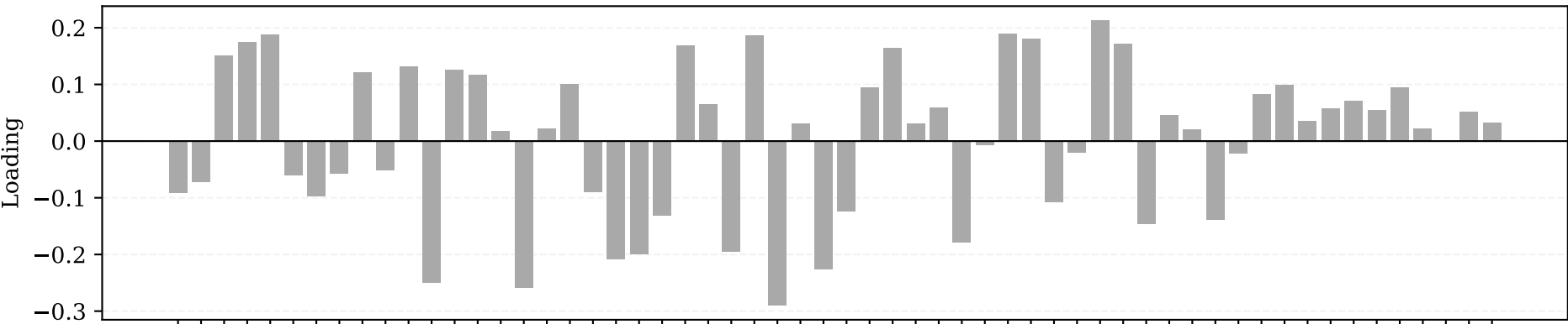
Eigenvector 5 ( \lambda = 1.48 ) | Dominant Sector: Utilities
