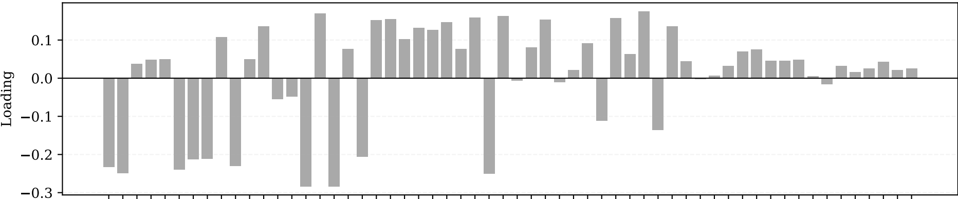
Eigenvector 2 ( \lambda = 3.10 ) | Dominant Sector: Basic Materials
