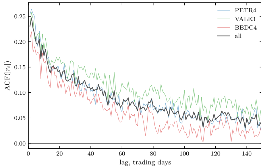
autocorrelations
