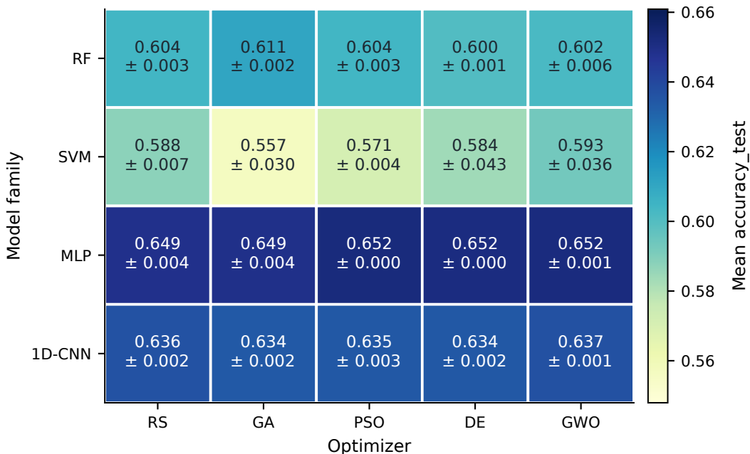
Weighted-accuracy fitness: Test-block accuracy
