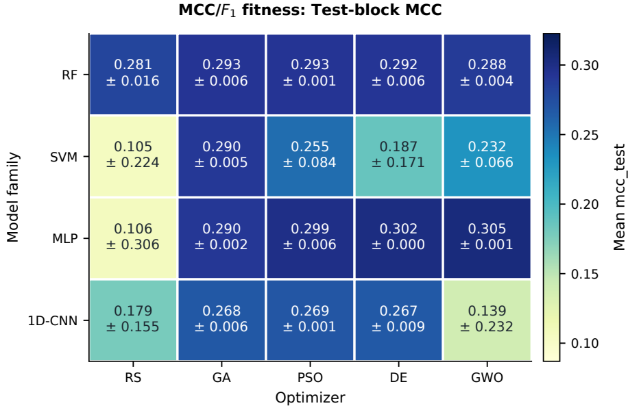
Fig. 18 Test-block MCC by classifier backbone and optimizer after selection under MCC/ F_1 fitness. Cells report the mean and standard deviation across the three common seeds; color encodes the mean.
