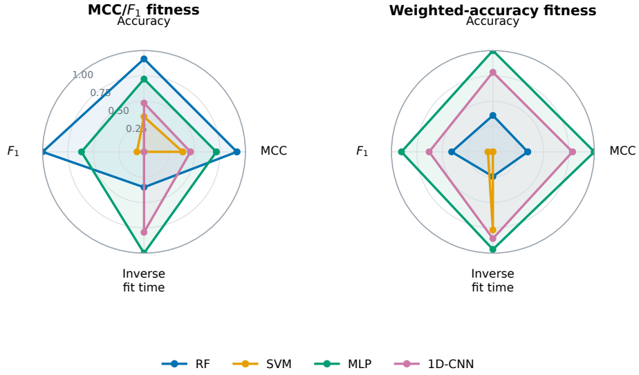
Fig. 22 Complementary normalized overview of test-block MCC, accuracy, F_1 , and inverse candidate-fit time by backbone and validation objective. Values are min–max normalized across the eight backbone–protocol averages; higher values indicate better values on each axis. Candidate-fit time is log-transformed before inversion and normalization.
