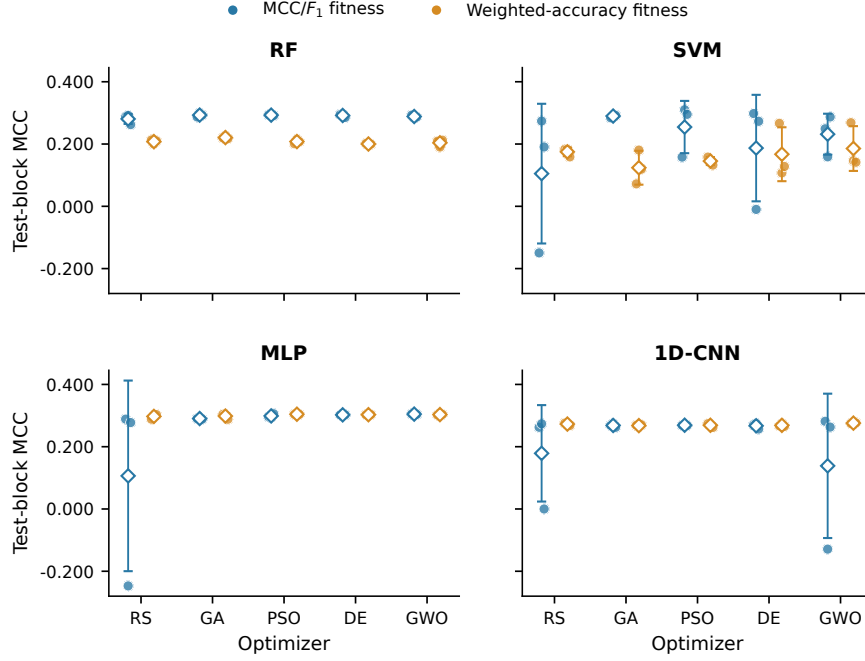
Fig. 20 Test-block MCC by optimizer and backbone under MCC/F_1 and weighted-accuracy fitness. Facets show the four backbones; points are the three common seed-level outcomes, and diamonds with vertical bars show the mean and one standard deviation. With three observations per cell, the display is descriptive rather than inferential.
