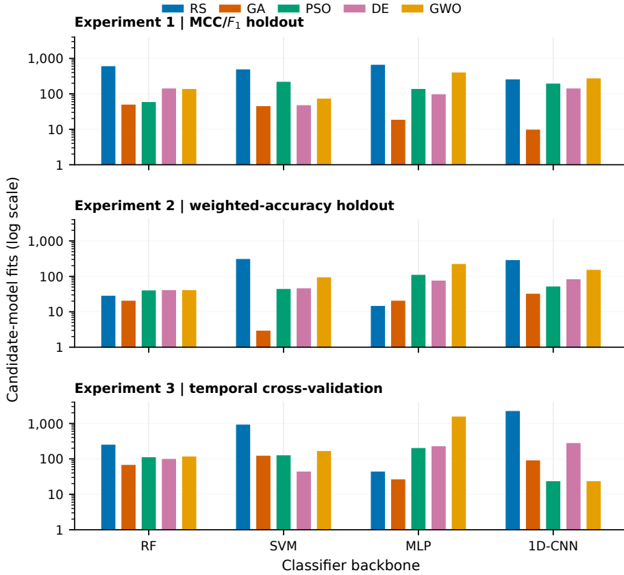
Fig. 16 Practical search effort measured as the median number of uncached candidate-model fits needed to reach 95% of each run’s own validation-fitness gain. This threshold is computed from validation fitness and is not a test-performance target. Bars are grouped by backbone and optimizer; panels show the two holdout protocols and exploratory temporal cross-validation. The vertical axis is logarithmic. Experiment 3 counts one model fit per fold (three per uncached candidate). Lower bars indicate fewer fits to that run’s own relative threshold, not fewer fits to attain a common absolute fitness.
