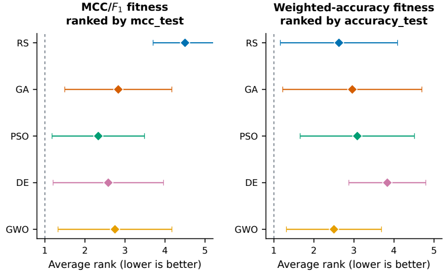
Fig. 21 Descriptive average ranks of the five optimizers across 12 backbone–seed combinations (four backbones and three common seeds). Rankings use test-block MCC under MCC/ F_1 fitness and test-block accuracy under weighted-accuracy fitness. Error bars show one standard deviation of block-level ranks; lower ranks indicate better ordering. This plot is descriptive and does not represent an optimizer significance test.
