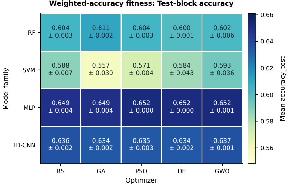
Fig. 19 Test-block accuracy by classifier backbone and optimizer after selection under weighted-accuracy fitness. Cells report the mean and standard deviation across the three common seeds; color encodes the mean.
