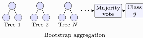
(a) Random Forest
