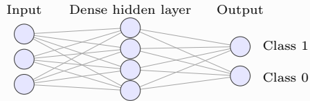
(c) Multilayer Perceptron
