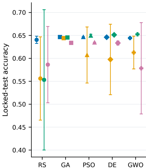
Exp. 1 | MCC/ F_1 fitness
