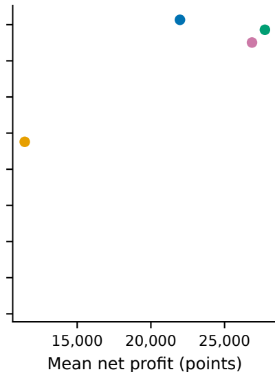
Weighted-accuracy fitness
