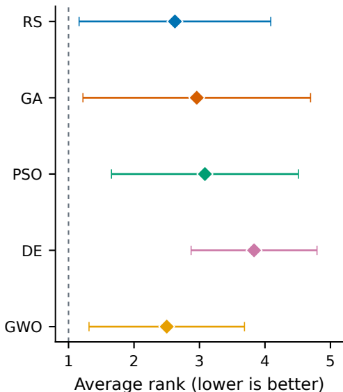
Weighted-accuracy fitness ranked by accuracy_test
