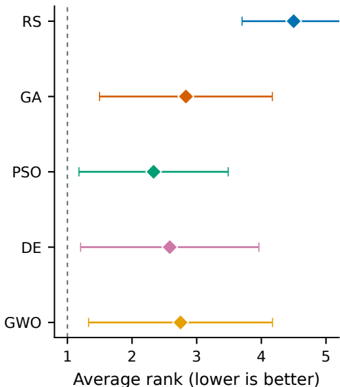
MCC/ F_1 fitness ranked by mcc_test
