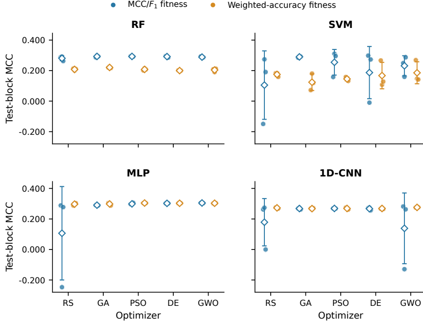
Fig. 19 Test-block MCC by optimizer and backbone under MCC/ F_1 and weighted-accuracy fitness. Facets show the four backbones; points are the three common seed-level outcomes, and diamonds with vertical bars show the mean and one standard deviation. With three observations per cell, the display is descriptive rather than inferential.
