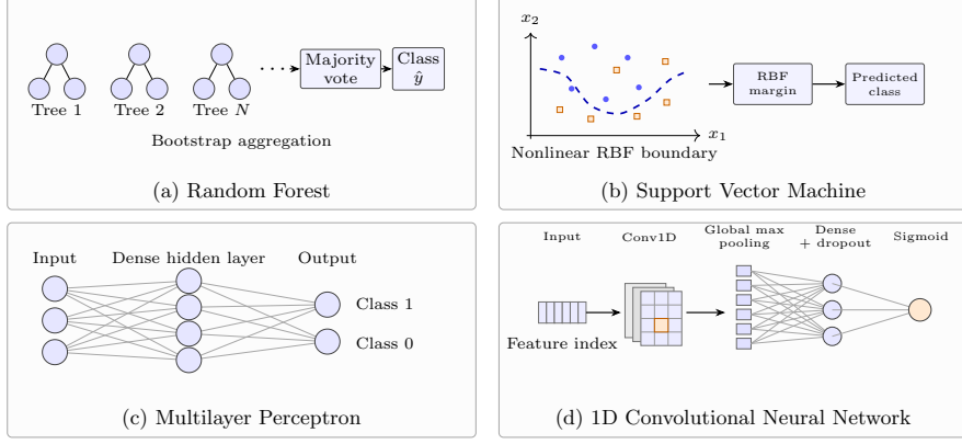
Fig. 4 Architectural topologies and structural decision mechanisms of the four candidate classifier backbones evaluated under the equal-budget metaheuristic optimization framework.
