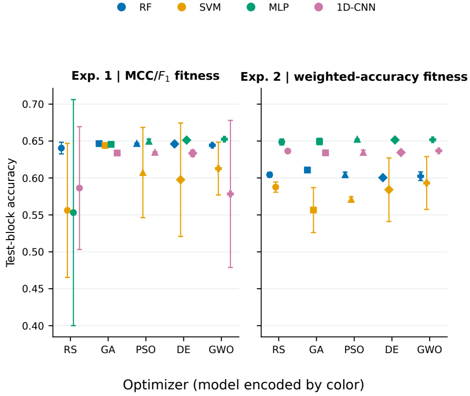
Fig. 14 Test-block accuracy under the two temporal holdout experiments. Experiment 1 selects with MCC/ F_1 fitness and Experiment 2 with weighted-accuracy fitness. Points show means and error bars show standard deviations across three common seeds; color identifies the backbone.
