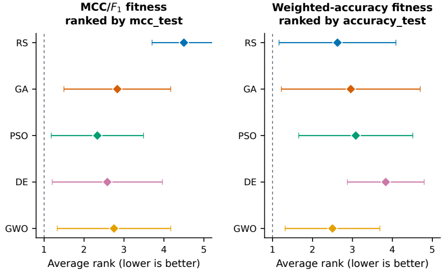
Fig. 20 Descriptive average ranks of the five optimizers across 12 backbone-seed combinations (four backbones and three common seeds). Rankings use test-block MCC under MCC/ F_1 fitness and test-block accuracy under weighted-accuracy fitness. Error bars show one standard deviation of block-level ranks; lower ranks indicate better ordering. This plot is descriptive and does not represent an optimizer significance test.
