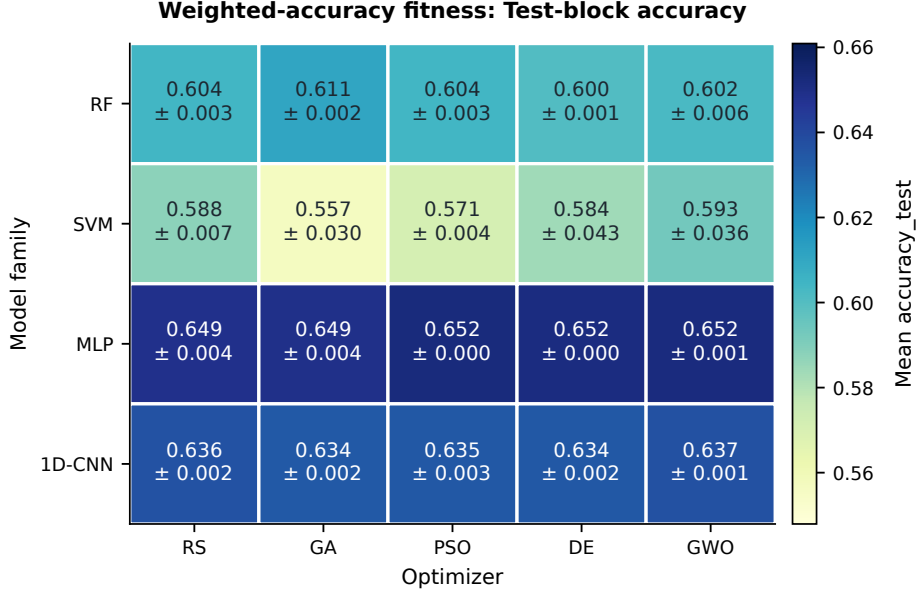
Fig. 18 Test-block accuracy by classifier backbone and optimizer after selection under weighted-accuracy fitness. Cells report the mean and standard deviation across the three common seeds; color encodes the mean.
