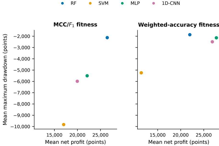
Fig. 16 Mean next-bar net profit versus mean maximum drawdown by backbone under \text{MCC}/F_1 and weighted-accuracy fitness. Each signal enters at the next five-minute bar open and exits at its close; values aggregate 15 optimizer–seed blocks. Both axes are in points, and a drawdown closer to zero indicates a smaller peak-to-trough loss.
