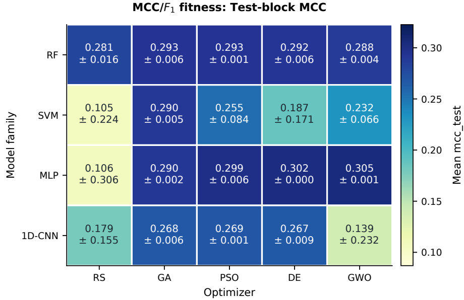
Fig. 17 Test-block MCC by classifier backbone and optimizer after selection under MCC/ F_1 fitness. Cells report the mean and standard deviation across the three common seeds; color encodes the mean.
