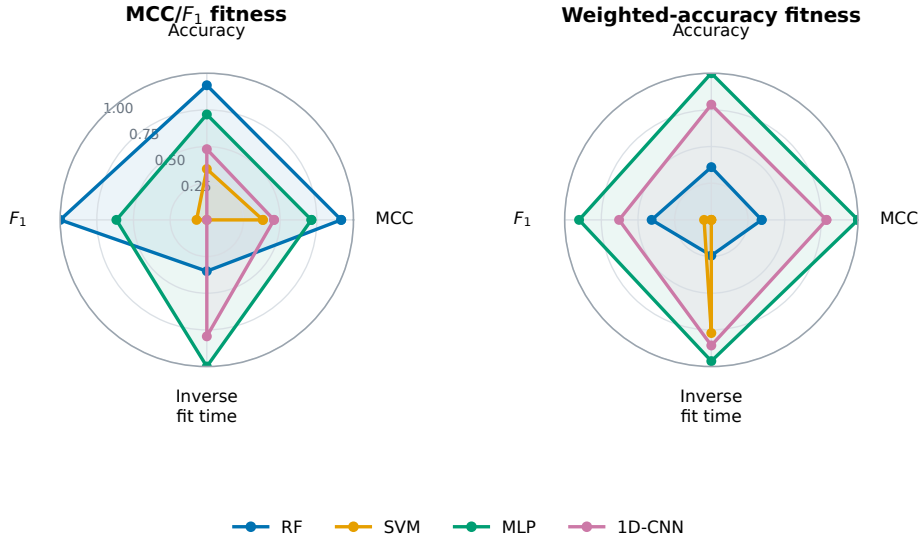
Fig. 21 Complementary normalized overview of test-block MCC, accuracy, F_1 , and inverse candidate-fit time by backbone and validation objective. Values are min-max normalized across the eight backbone-protocol averages; higher values indicate better values on each axis. Candidate-fit time is log-transformed before inversion and normalization.
