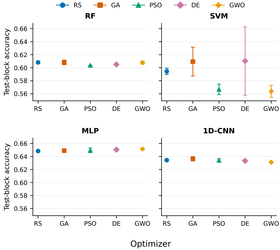
Fig. 15 Test-block accuracy after configuration selection with the weighted-accuracy objective under three-fold temporal cross-validation (Experiment 3). Points show means and error bars show standard deviations across three common seeds for each optimizer and backbone.
