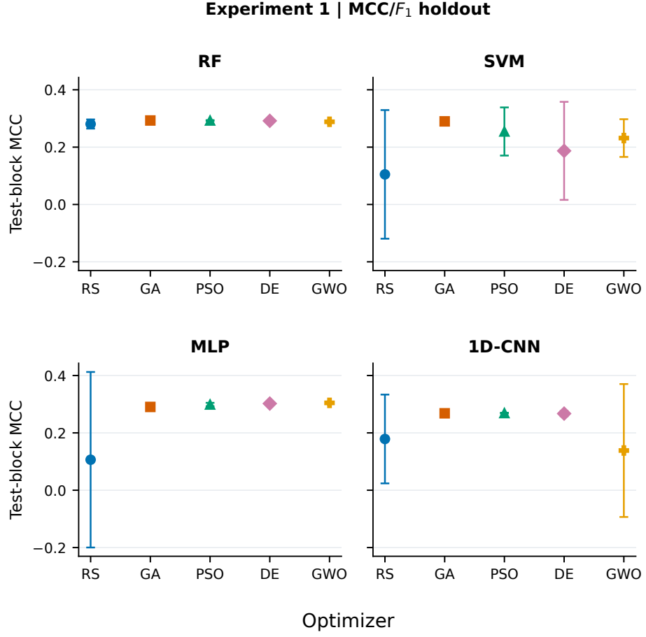
Fig. 13 Test-block MCC for Experiment 1, which selects configurations using MCC/ F_1 fitness under temporal holdout. Points show means and error bars show standard deviations across three common seeds for each optimizer and backbone.
