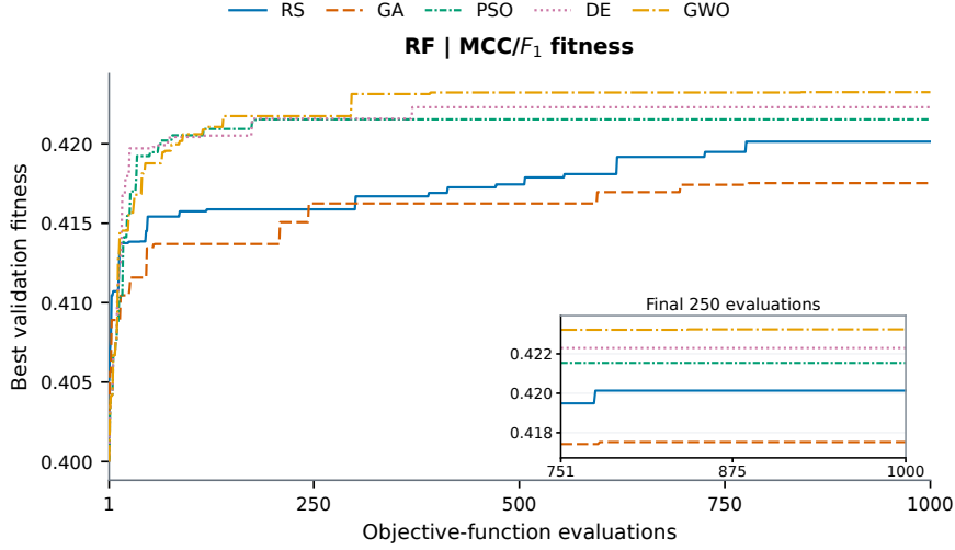
Fig. 5 Best-so-far validation fitness over 1,000 objective-function evaluations for RF under MCC/F_1 fitness. Curves show mean fitness across the three common seeds for RS, GA, PSO, DE, and GWO; the inset covers evaluations 751–1,000.
