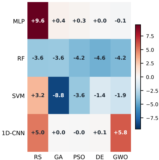
Delta test accuracy (percentage points)
