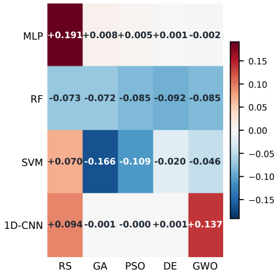
Delta test MCC
