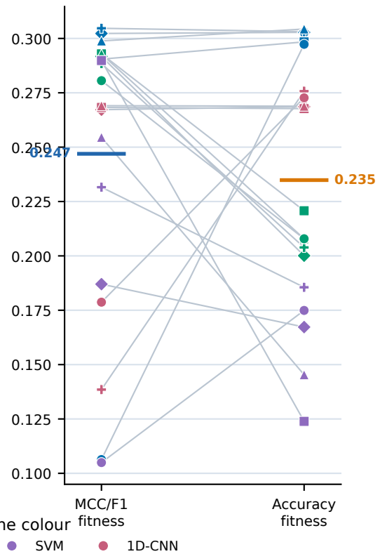
Test MCC
