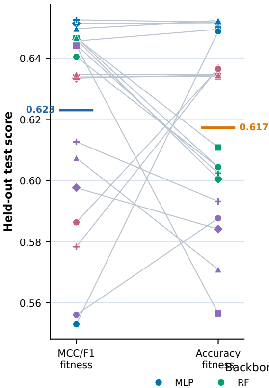
Test accuracy
