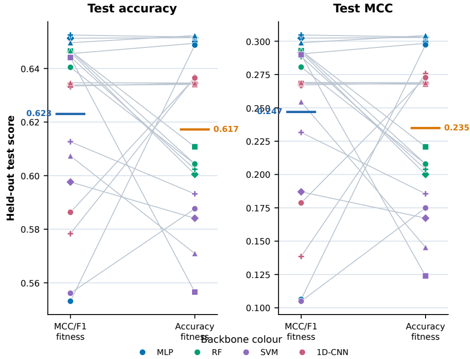
Fig. 3 Held-out performance under the two validation objectives. Each connected pair is the mean of the same three seeds for one model-optimizer cell; colour identifies the backbone and marker shape identifies the optimizer. Short horizontal segments give the macro mean across the 20 cells.
