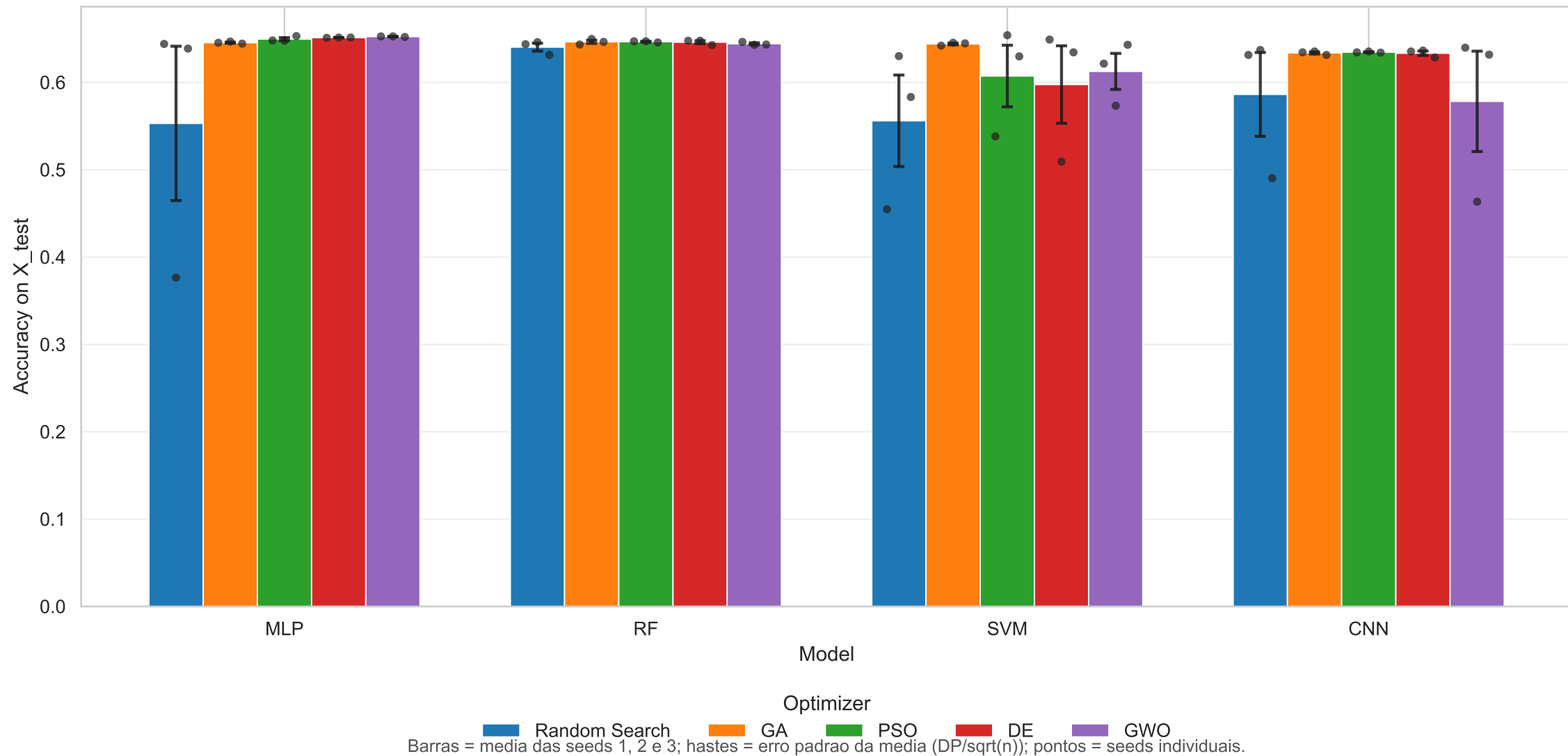
MCC/F1 fitness benchmark - Accuracy on X_test by model and optimizer
