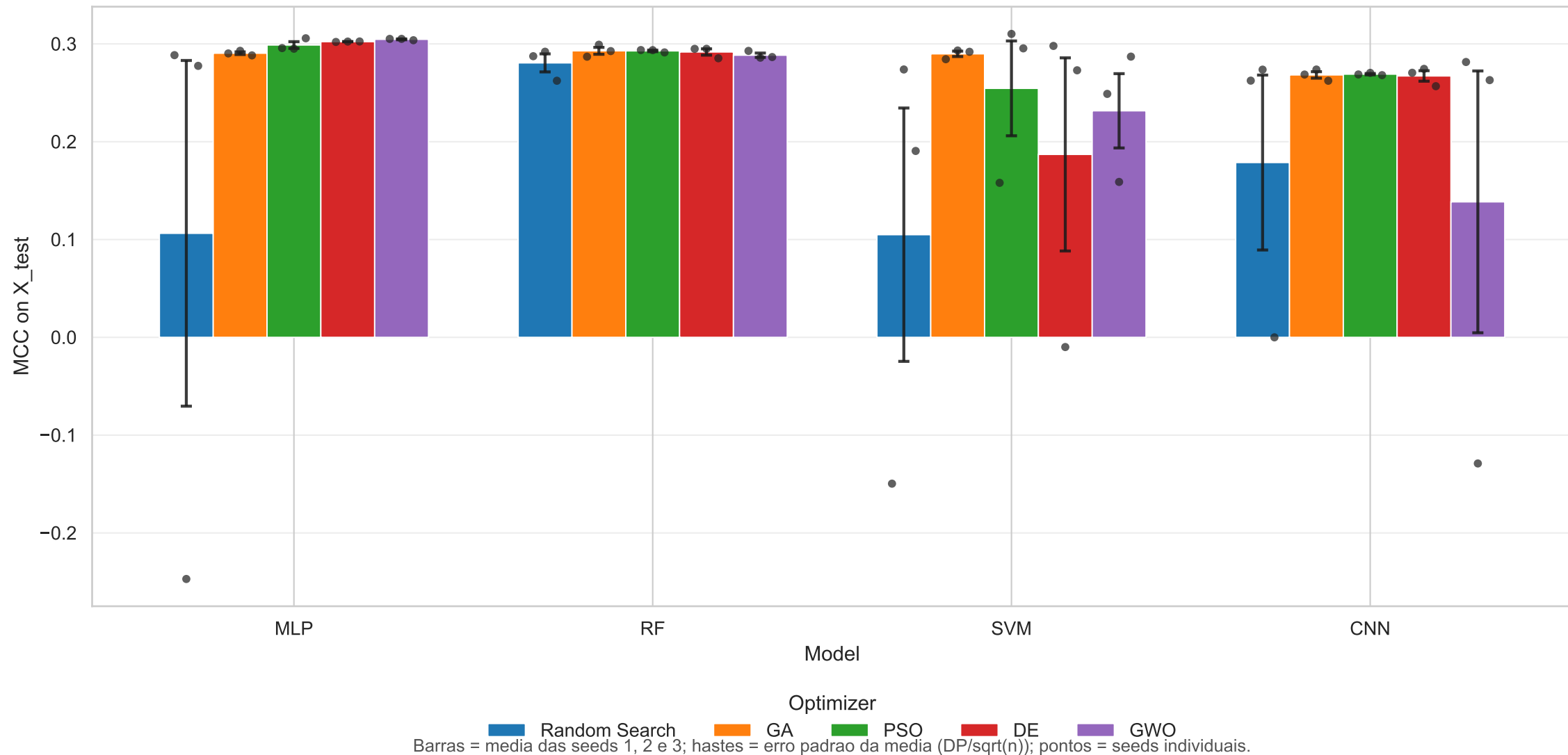
MCC/F1 fitness benchmark - MCC on X_test by model and optimizer
