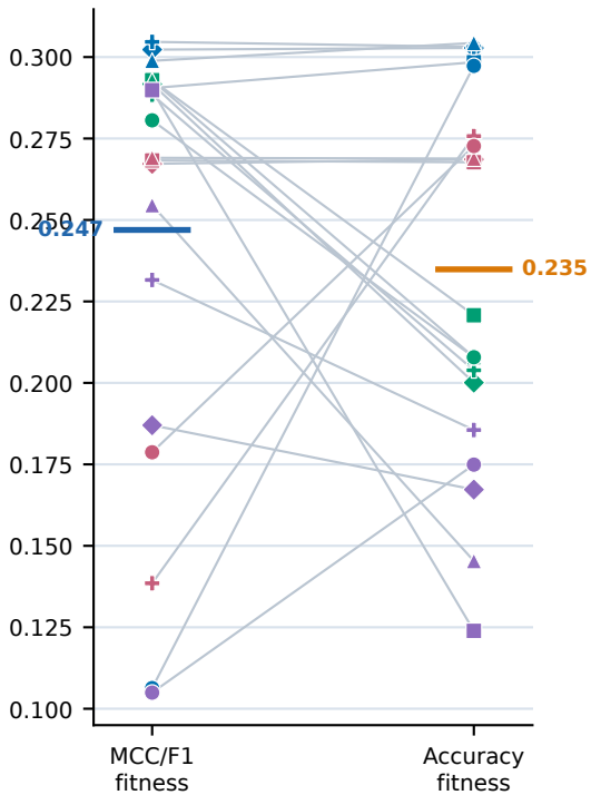
Test MCC
