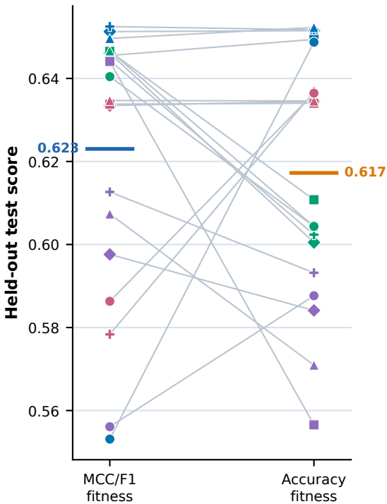
Test accuracy
