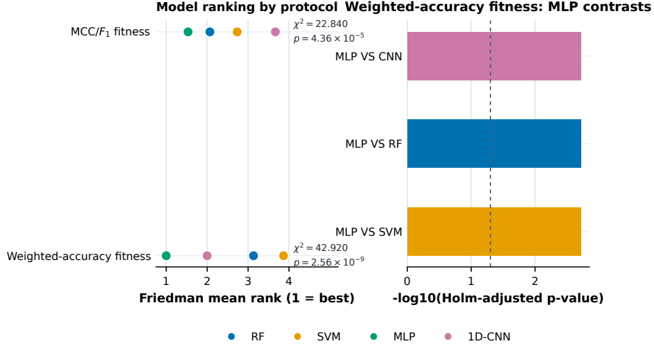
Fig. 17 Exploratory matched-block evidence for backbone comparisons. The left panel shows Friedman mean ranks on protocol-aligned locked-test endpoints across 15 optimizer–seed blocks (lower is better); the right panel shows -\log_{10} Holm-adjusted p -values for weighted-accuracy contrasts against MLP, with the vertical line marking \alpha = 0.05 .
