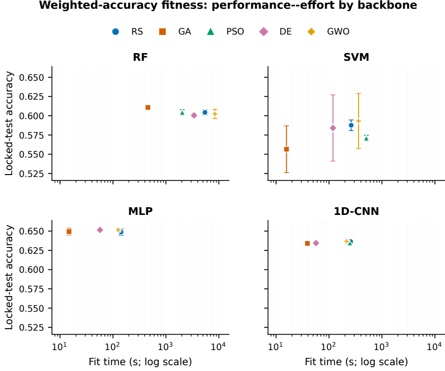
Fig. 24 Locked-test accuracy versus mean cumulative uncached candidate-fit time under weighted-accuracy fitness. Separate panels show the four backbones; color and marker identify the optimizer. Points are means across three common seeds, with vertical bars indicating one standard deviation in test accuracy. The horizontal axis is logarithmic and sums recorded fit times across candidates; it is not end-to-end optimizer wall-clock time.
