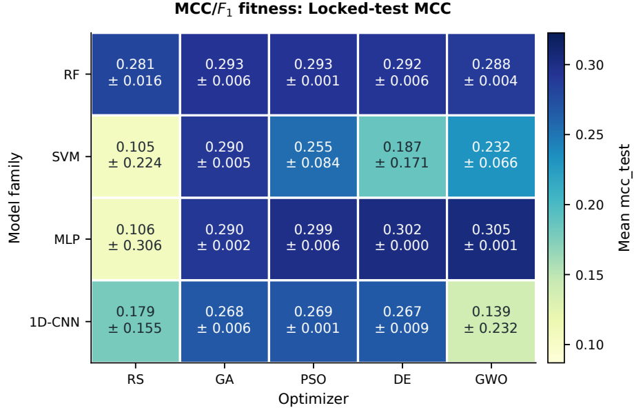
Fig. 19 Locked-test MCC by classifier backbone and optimizer after selection under MCC/ F_1 fitness. Cells report the mean and standard deviation across the three common seeds; color encodes the mean.
