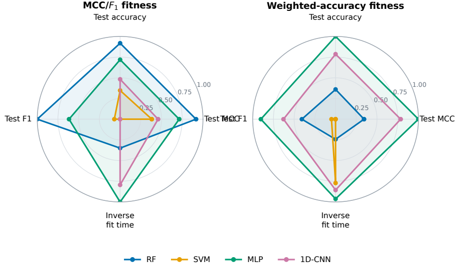
Fig. 25 Complementary normalized overview of locked-test MCC, accuracy, F_1 , and inverse candidate-fit time by backbone and validation objective. Values are min-max normalized across the eight backbone-protocol averages; higher values indicate better values on each axis. Candidate-fit time is log-transformed before inversion and normalization.
