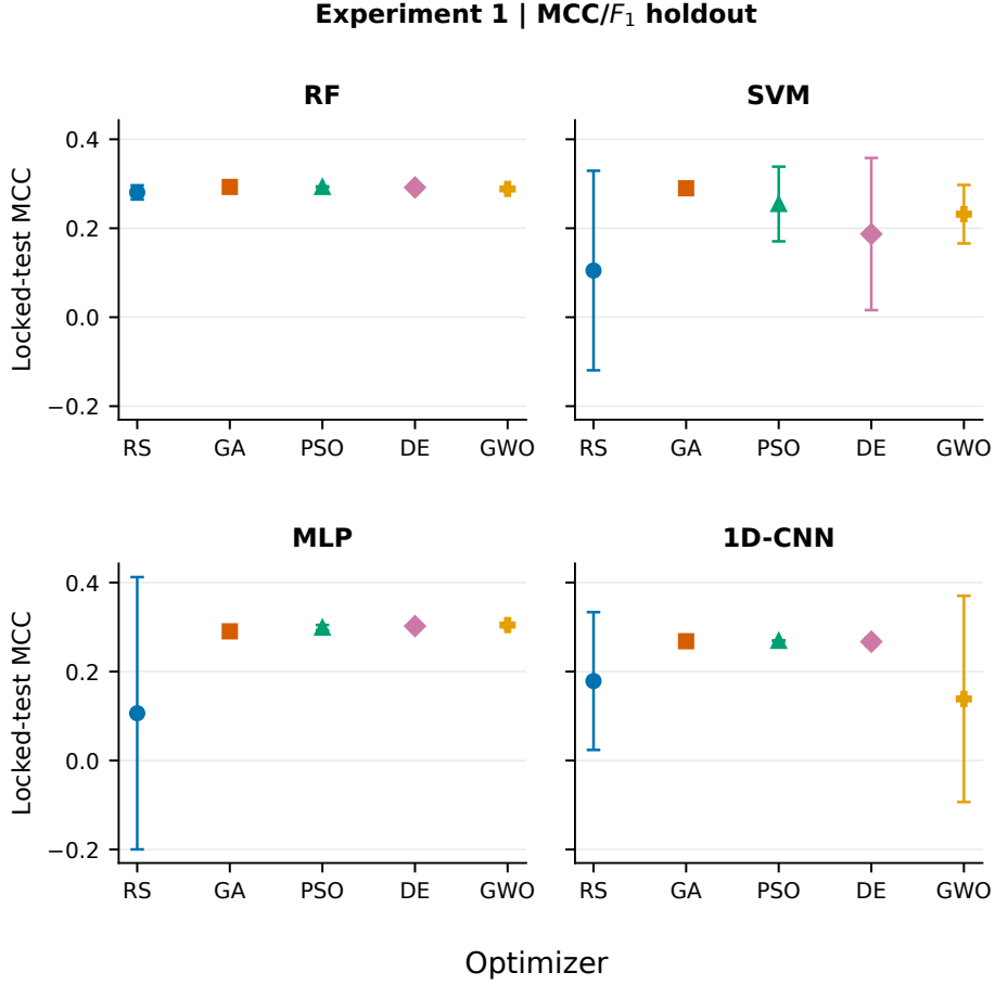
Fig. 14 Locked-test MCC for Experiment 1, which selects configurations using MCC/ F_1 fitness under temporal holdout. Points show means and error bars show standard deviations across three common seeds for each optimizer and backbone.
