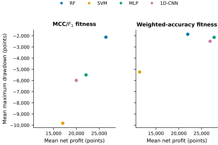
Fig. 18 Mean net profit versus mean maximum drawdown by backbone under MCC/ F_1 and weighted-accuracy fitness. Values aggregate 15 optimizer–seed blocks; both axes are in points, and a drawdown closer to zero indicates a smaller peak-to-trough loss.
