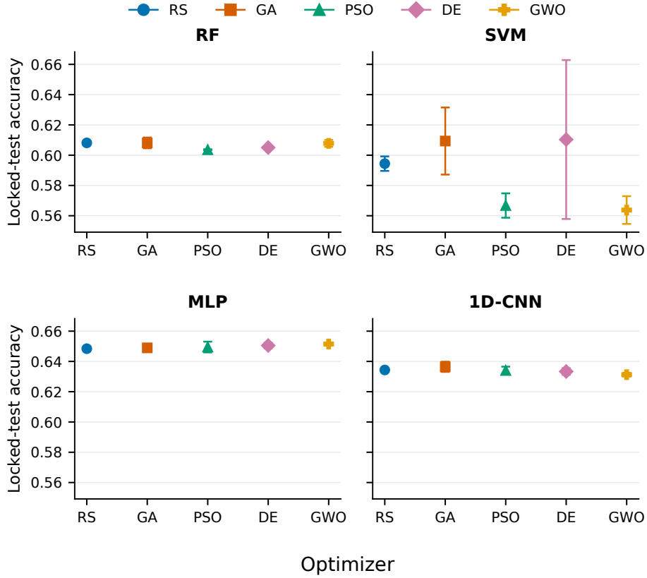
Fig. 16 Locked-test accuracy after configuration selection with the weighted-accuracy objective under three-fold temporal cross-validation (Experiment 3). Points show means and error bars show standard deviations across three common seeds for each optimizer and backbone.
