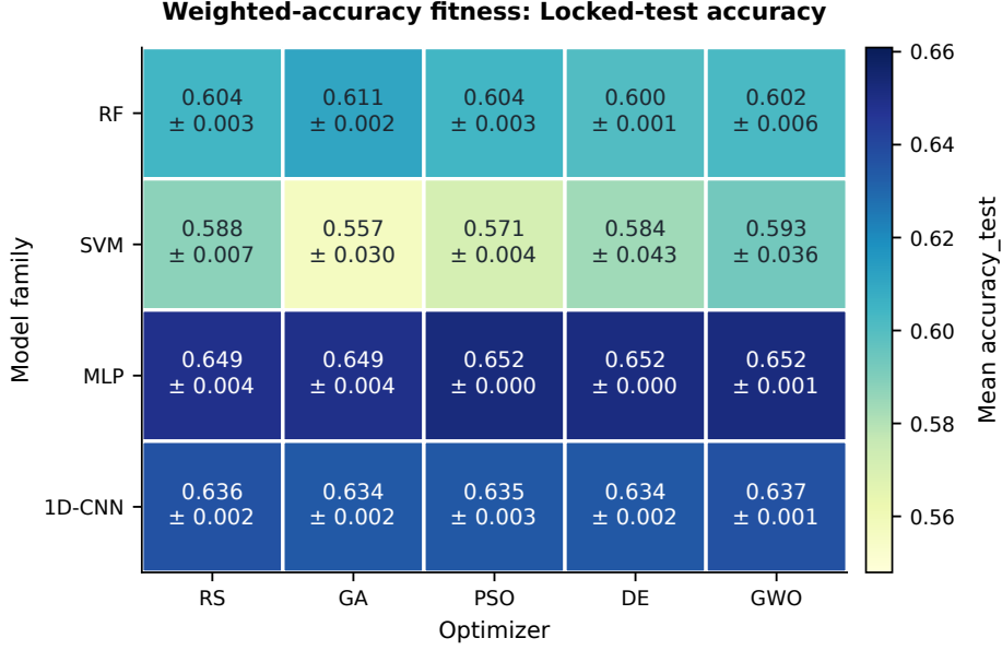
Fig. 20 Locked-test accuracy by classifier backbone and optimizer after selection under weighted-accuracy fitness. Cells report the mean and standard deviation across the three common seeds; color encodes the mean.
