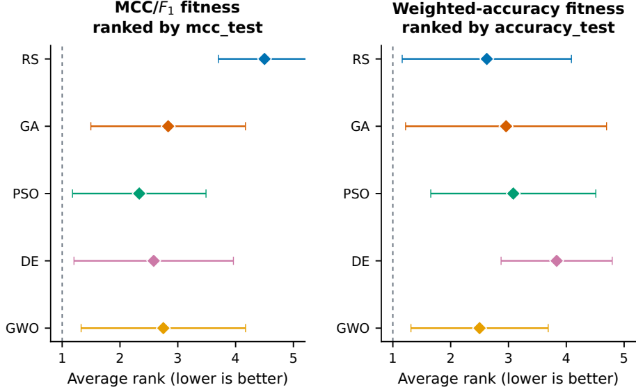
Fig. 22 Descriptive average ranks of the five optimizers across 12 backbone-seed combinations (four backbones and three common seeds). Rankings use locked-test MCC under MCC/ F_1 fitness and locked-test accuracy under weighted-accuracy fitness. Error bars show one standard deviation of block-level ranks; lower ranks indicate better ordering. This plot is descriptive and does not represent an optimizer significance test.
