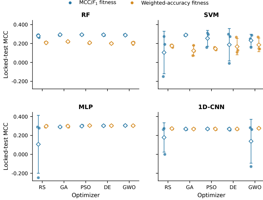
Fig. 21 Locked-test MCC by optimizer and backbone under MCC/ F_1 and weighted-accuracy fitness. Facets show the four backbones; points are the three common seed-level outcomes, and diamonds with vertical bars show the mean and one standard deviation. With three observations per cell, the display is descriptive rather than inferential.
