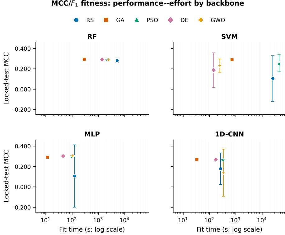
Fig. 23 Locked-test MCC versus mean cumulative uncached candidate-fit time under MCC/ F_1 fitness. Separate panels show the four backbones; color and marker identify the optimizer. Points are means across three common seeds, with vertical bars indicating one standard deviation in test MCC. The horizontal axis is logarithmic and sums recorded fit times across candidates; it is not end-to-end optimizer wall-clock time.
