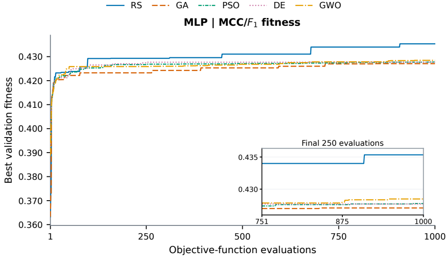
Fig. 10 Best-so-far validation fitness over 1,000 objective-function evaluations for MLP under \text{MCC}/F_1 fitness. Curves show mean fitness across the three common seeds for RS, GA, PSO, DE, and GWO; the inset covers evaluations 751–1,000.
