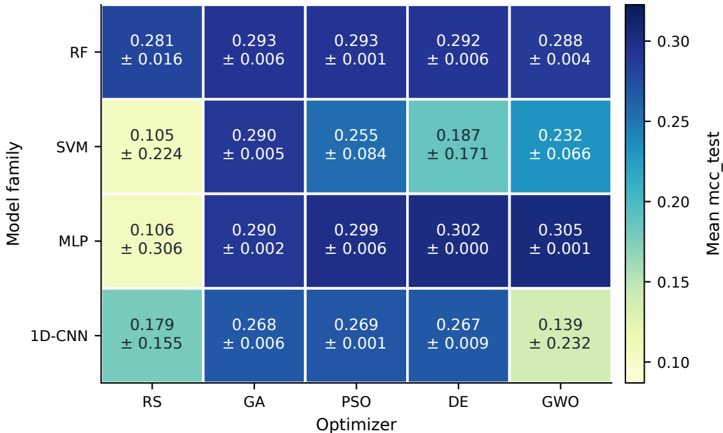
MCC/ F_1 fitness: Locked-test MCC
