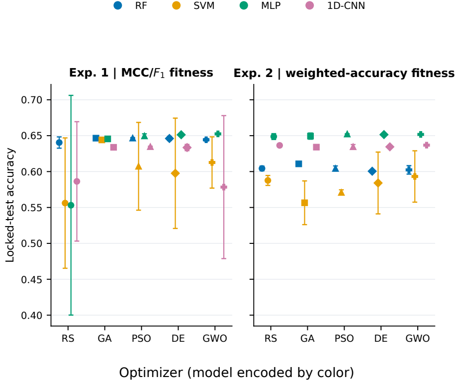
Fig. 15 Locked-test accuracy under the two temporal holdout experiments. Experiment 1 selects with \text{MCC}/F_1 fitness and Experiment 2 with weighted-accuracy fitness. Points show means and error bars show standard deviations across three common seeds; color identifies the backbone.
