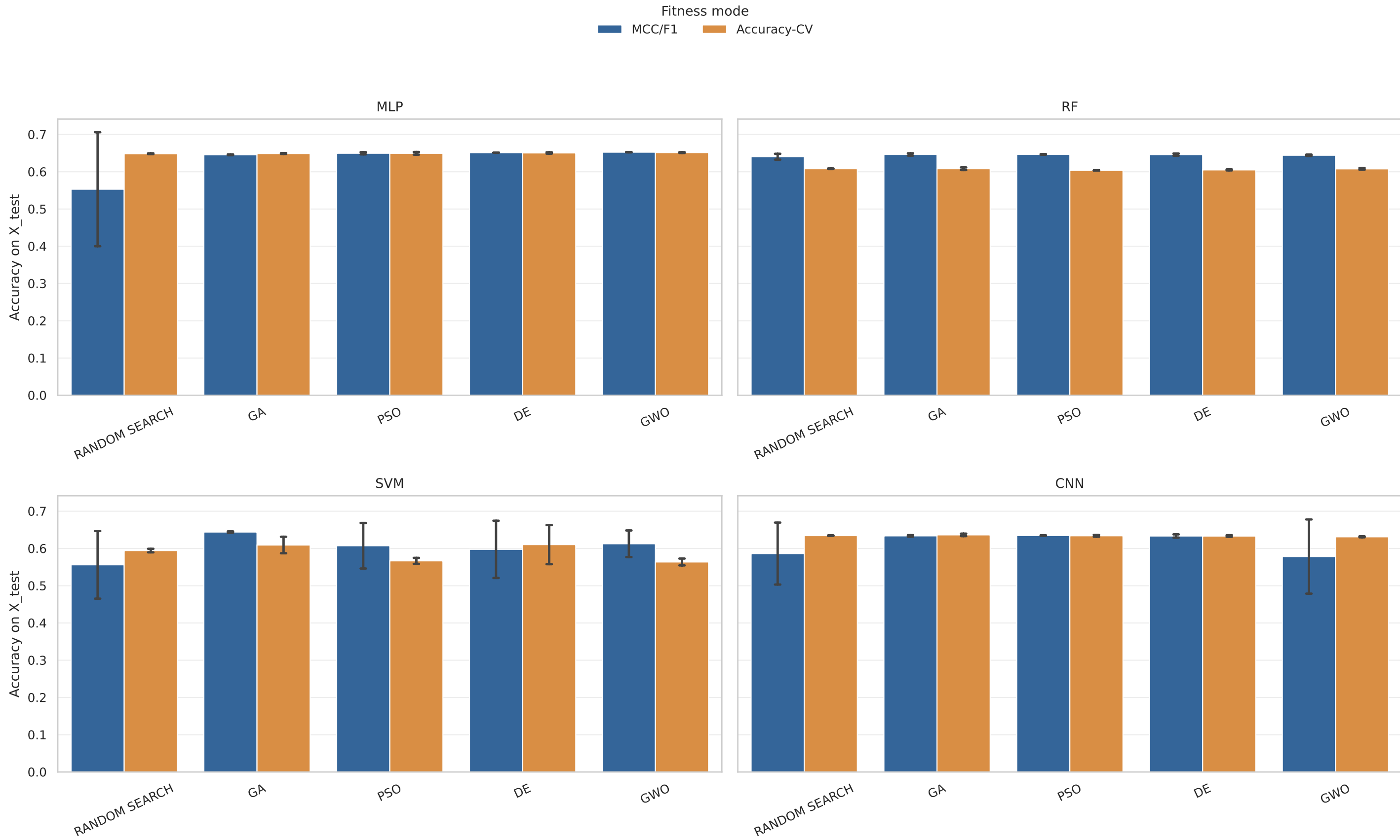
Accuracy on X_test by model, optimizer, and fitness mode
