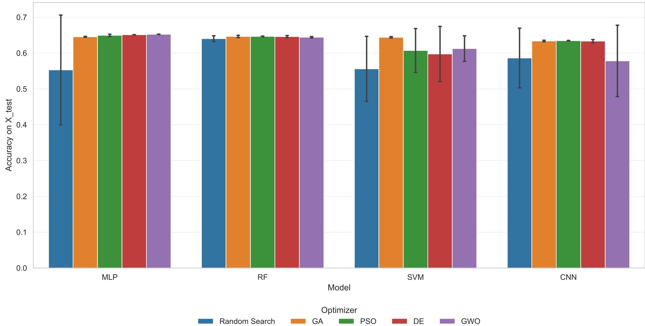
MCC/F1 fitness benchmark - Accuracy on X_test by model and optimizer
