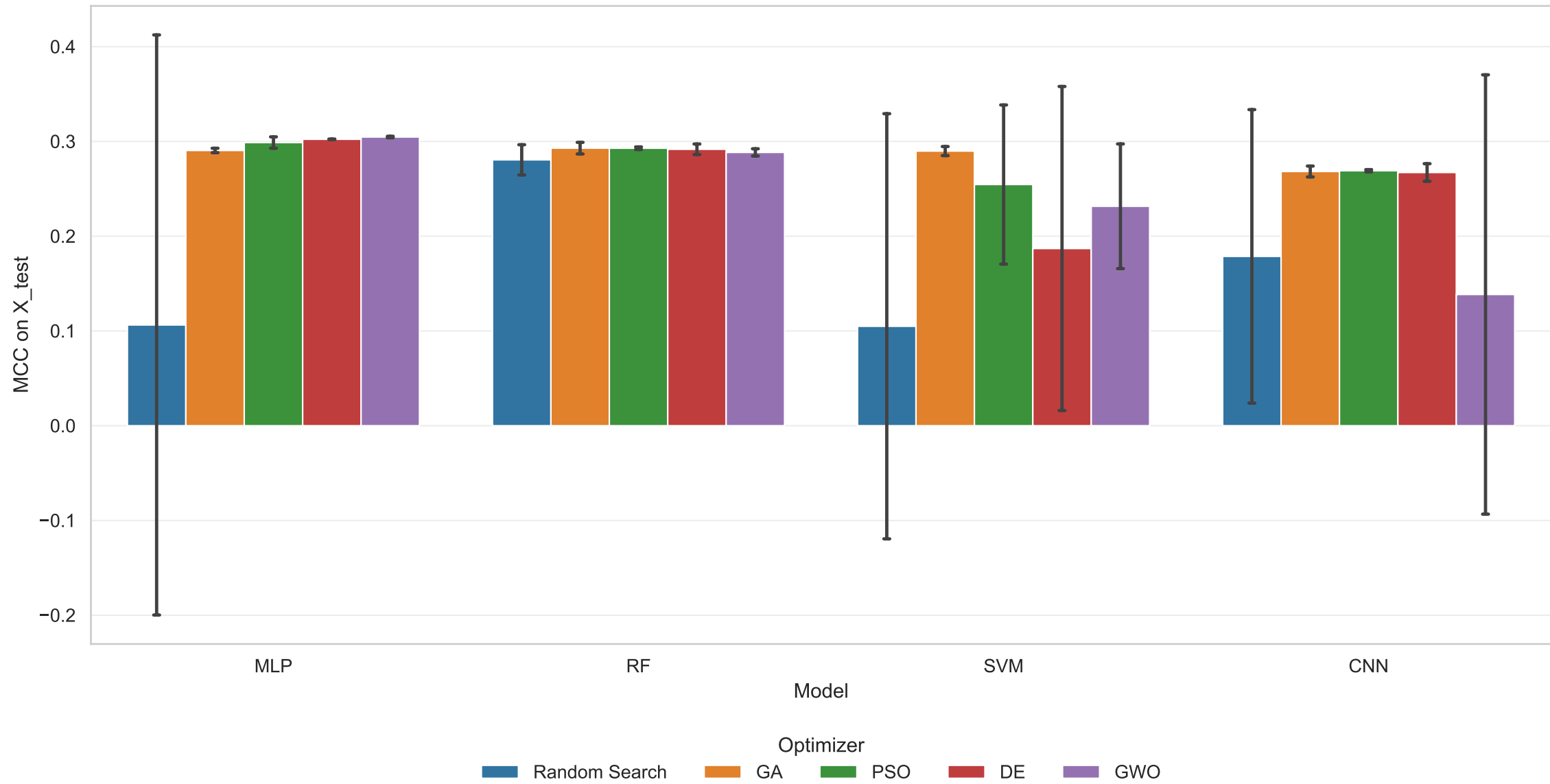
MCC/F1 fitness benchmark - MCC on X_test by model and optimizer
