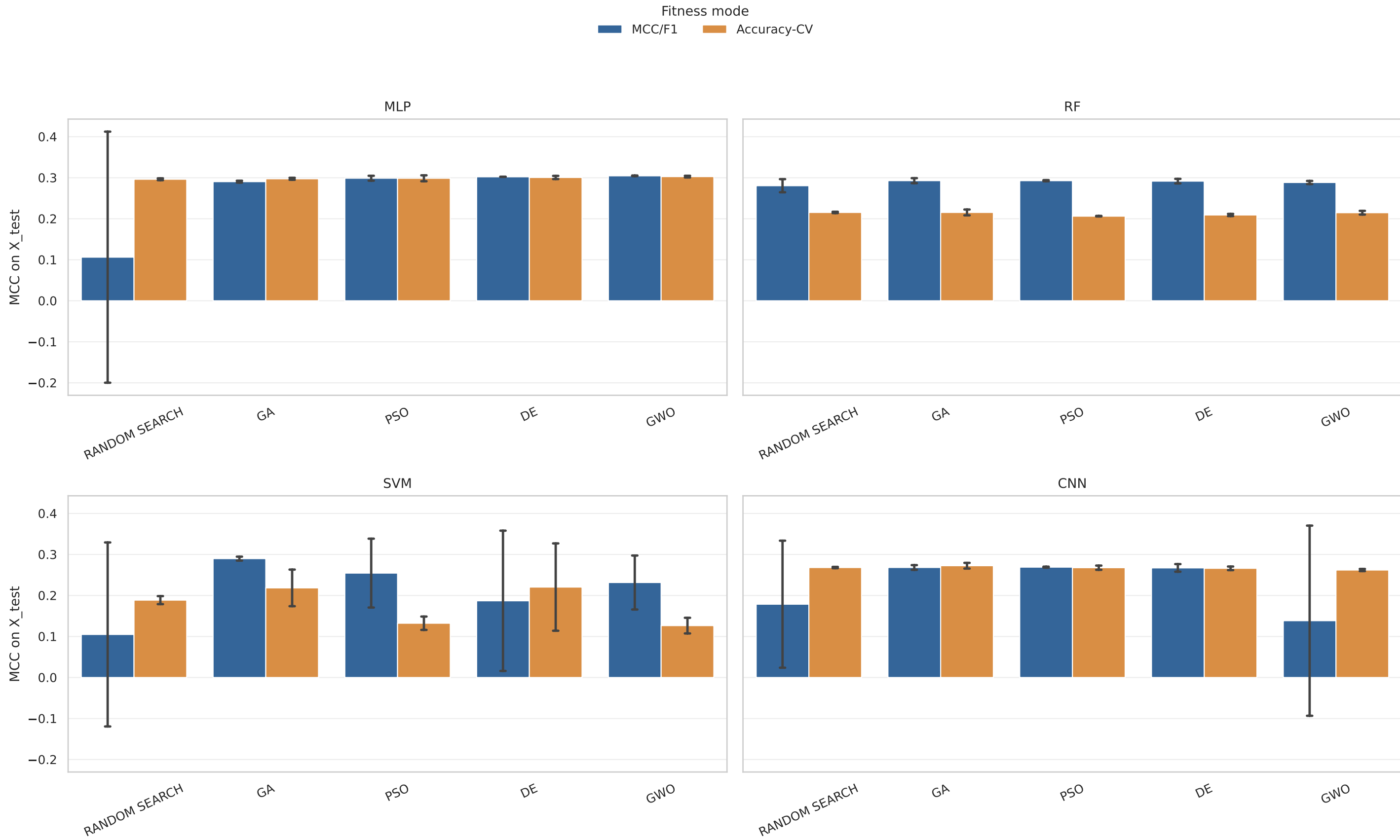
MCC on X_test by model, optimizer, and fitness mode
