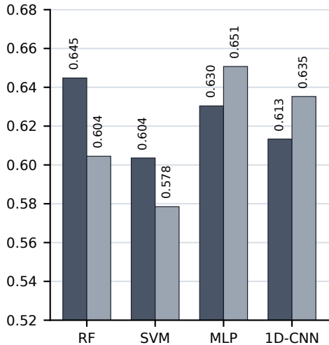
Held-out test accuracy
