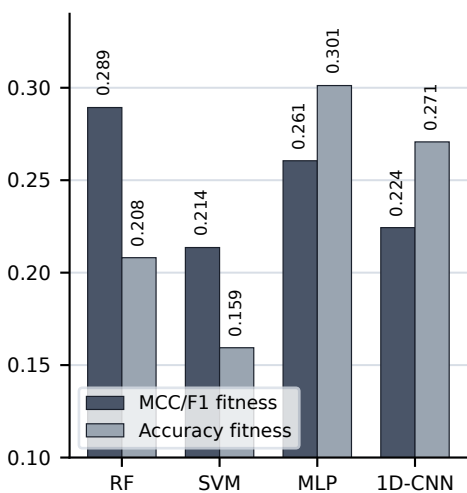
Held-out test MCC
