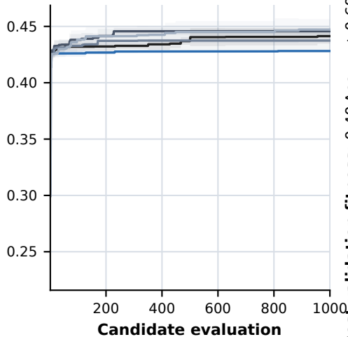
MCC/F1 fitness
