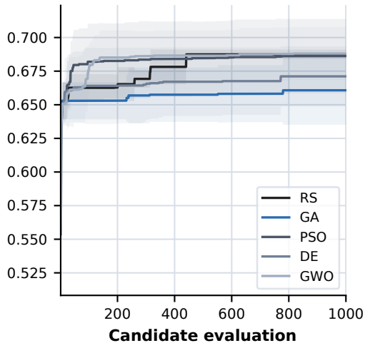
Accuracy fitness
