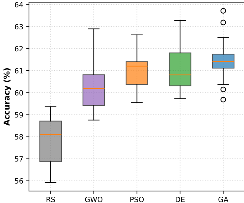
Out-of-Sample Accuracy (%)
