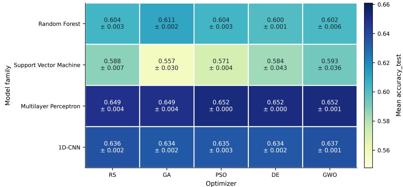
Weighted-accuracy objective: Locked-test accuracy
