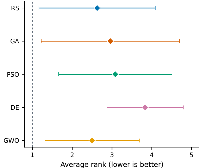
Weighted-accuracy objective ranked by accuracy_test
