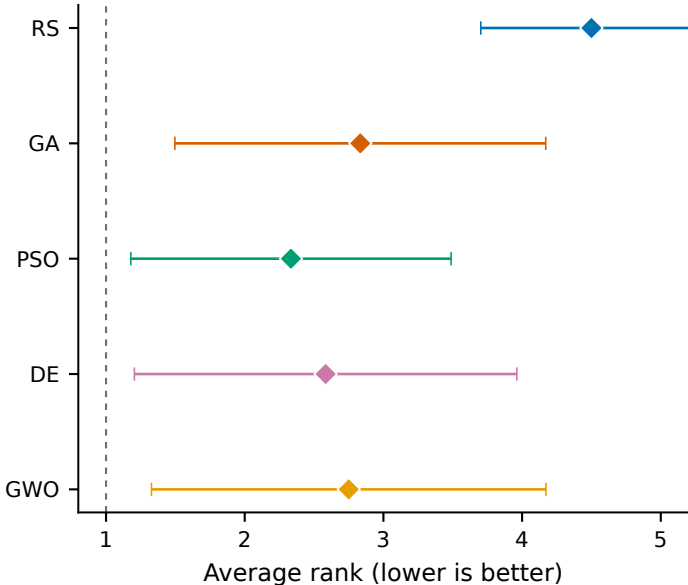
MCC/F1 objective ranked by mcc_test
