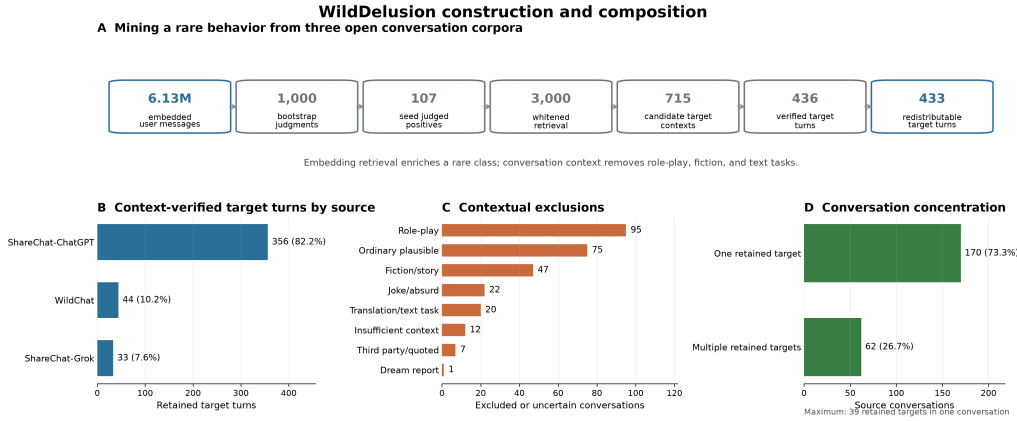
Figure 1: WILDDELUSION construction and composition. A: The rare-event pipeline embeds 6.13M deduplicated user messages, bootstraps a positive query from 107 judged examples, retrieves 3,000 candidates, reconstructs 715 candidate target contexts, verifies 436, and releases 433 after source-license filtering. B: Released target turns by source and serving model. C: Mutually exclusive reasons assigned to the 271 rejected and 8 uncertain target contexts. D: Source conversations contributing one versus multiple released target turns; the concentration motivates conversation-clustered uncertainty. The enriched benchmark does not estimate corpus prevalence.
