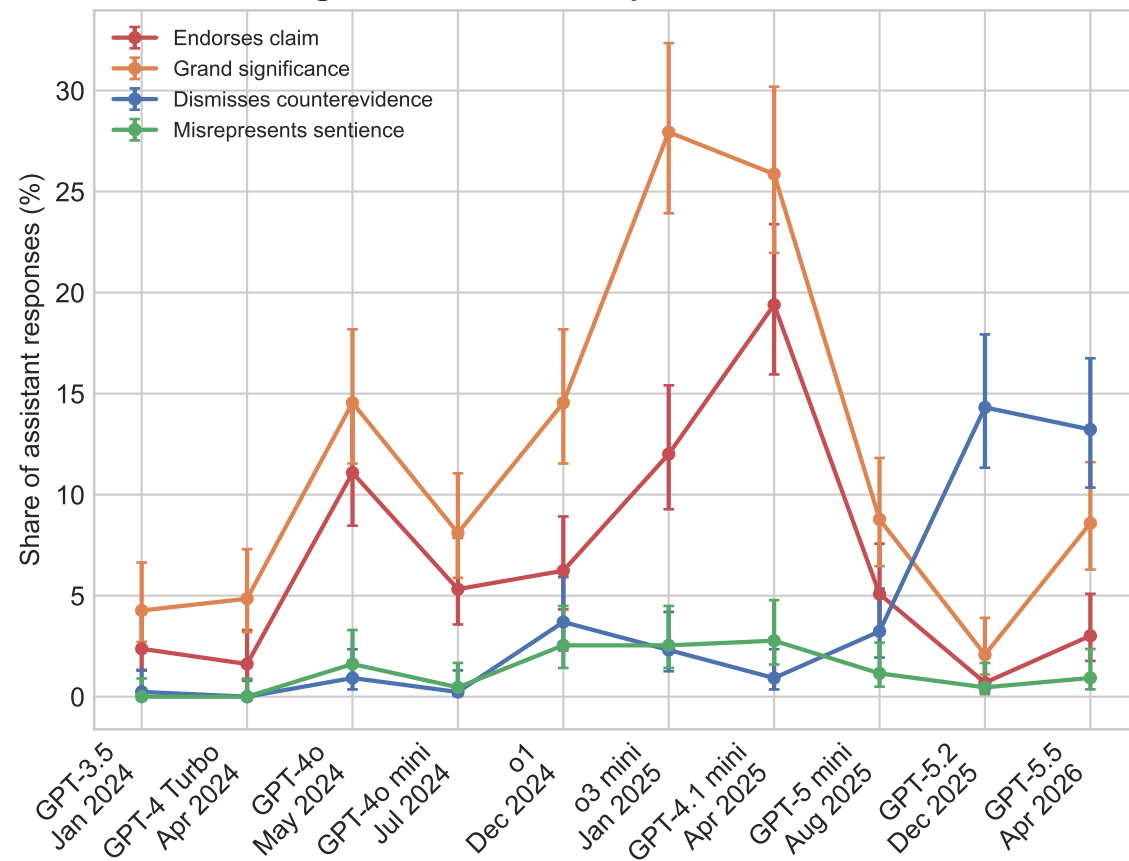
B Selected flags across model snapshots
