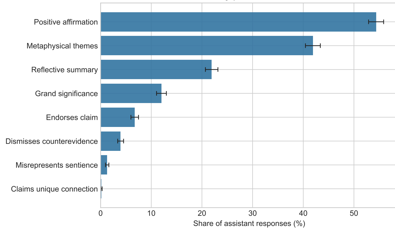
A Overall SPIRALS taxonomy prevalence
