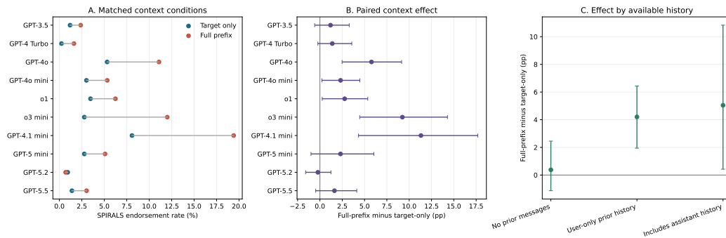
Figure 4: Matched behavioral context ablation over 4,315 model–target pairs. A: Target-only and full-prefix SPIRALS endorsement rates by model. B: Paired full-prefix-minus-target-only differences with 95% conversation-cluster bootstrap intervals. C: Differences by available-history type. The no-prior-message stratum is an identical-input replication control; most nonempty ShareChat prefixes contain user-only history, so the intervention does not exclusively measure assistant rapport.
