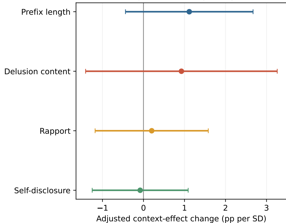
Adjusted heterogeneity
