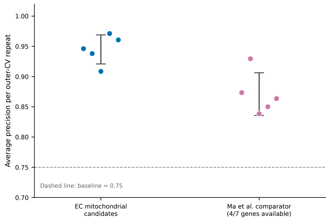
D Repeat-level average precision (mean \pm SD)
