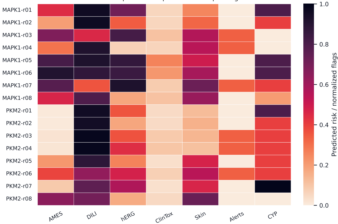
ADMET risk profile for top 8 candidates per target
