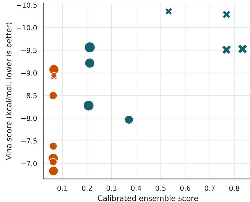
Docking support vs ligand-based score
