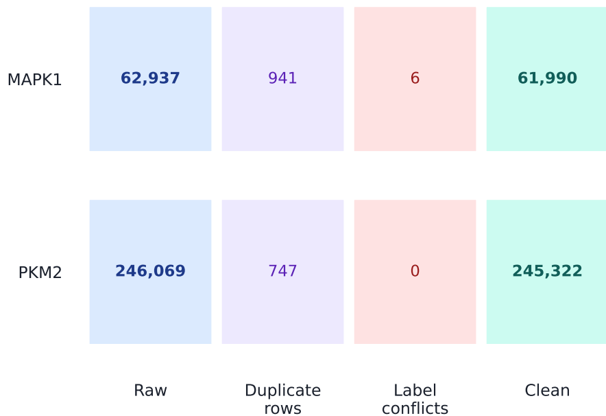
Curation flow
