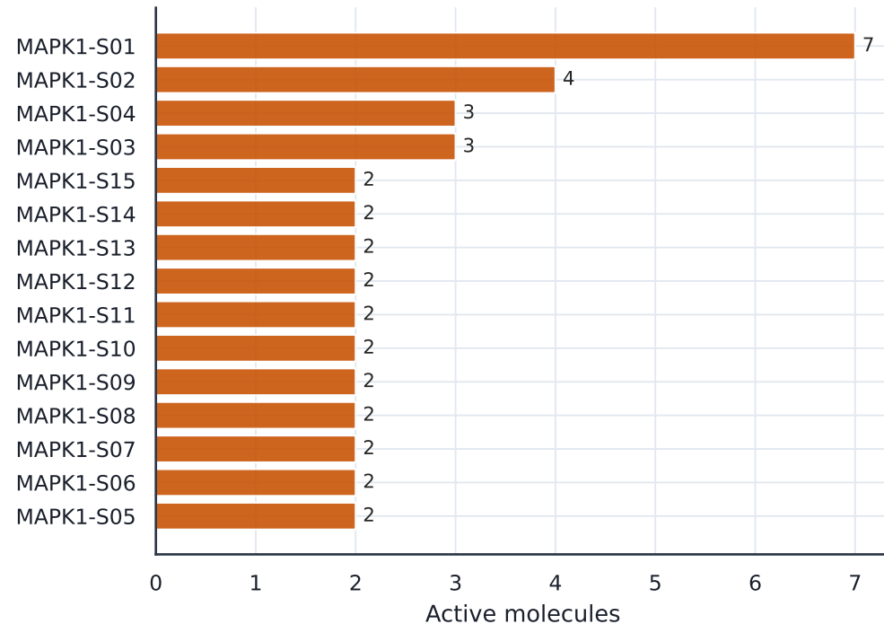
MAPK1: top active scaffolds
