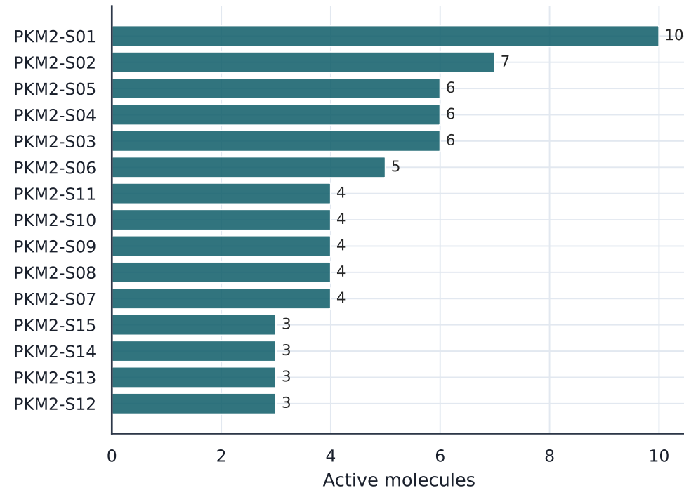
PKM2: top active scaffolds
