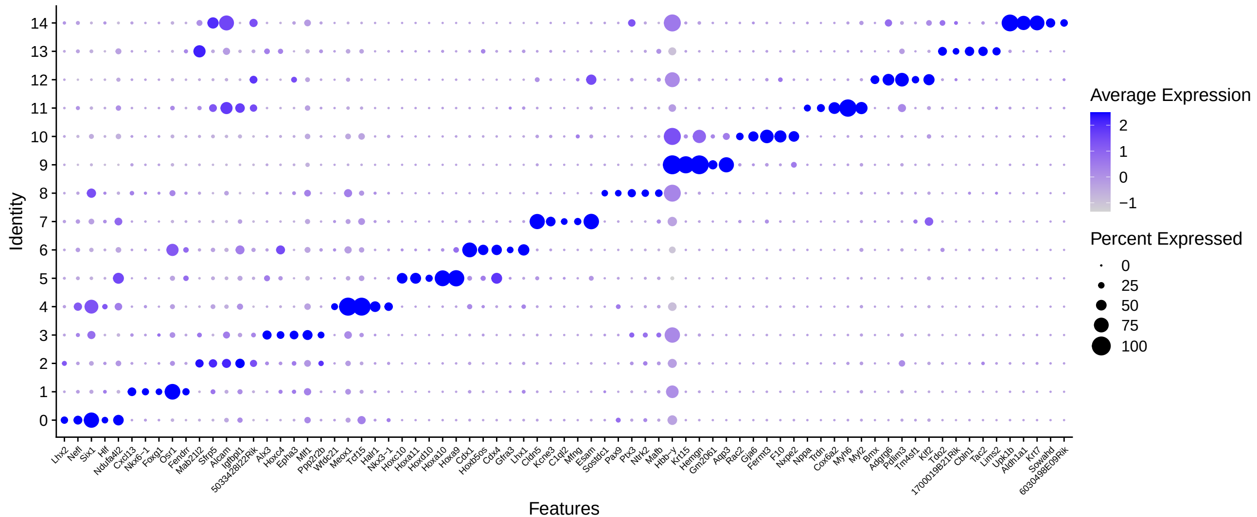
Top 5 data-driven markers / cluster (clust_res0.4)
